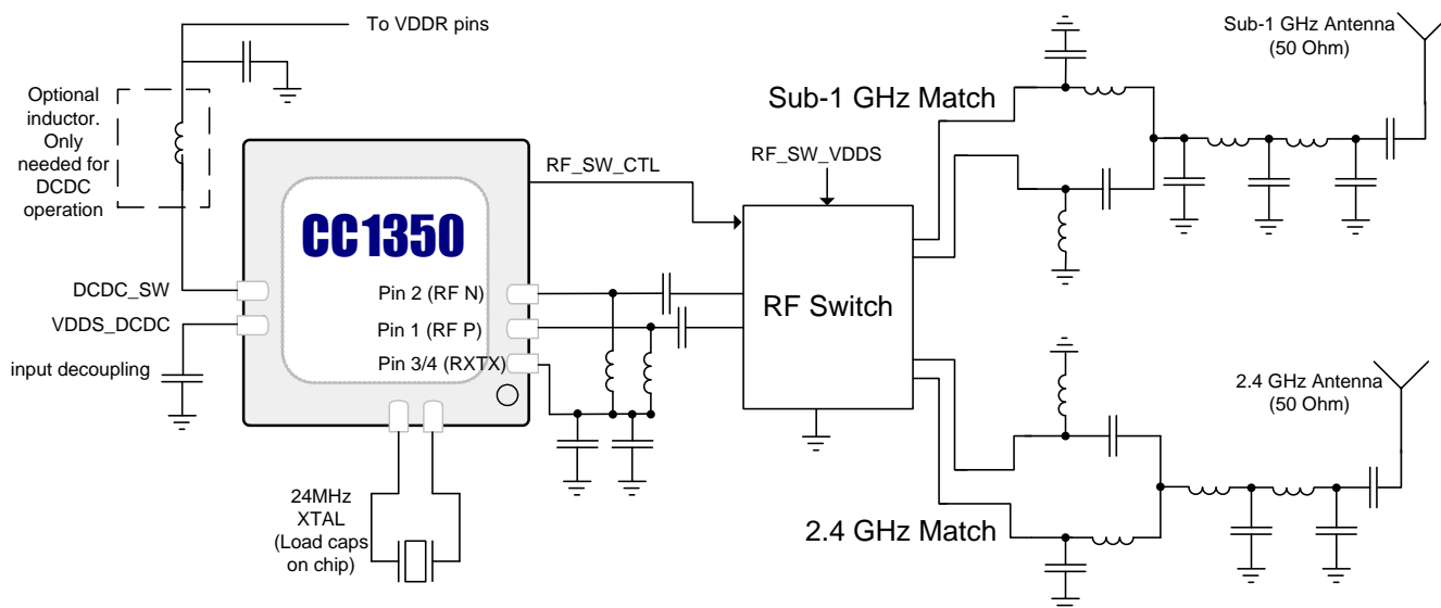
Figure 7-1 does not show decoupling capacitors for power pins. For a complete reference design, see the product folder on www.ti.com .
