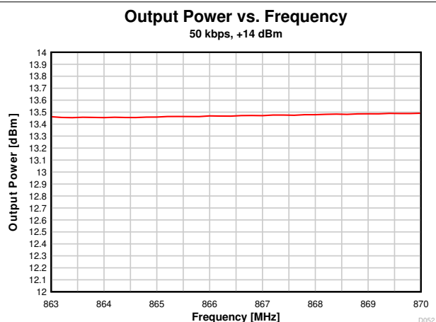
图 7-20. Output Power vs. Frequency (50 kbps, 868 MHz)
