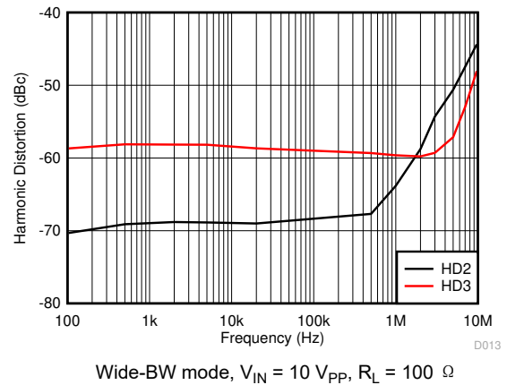
图 6-30. Harmonic Distortion vs Frequency
