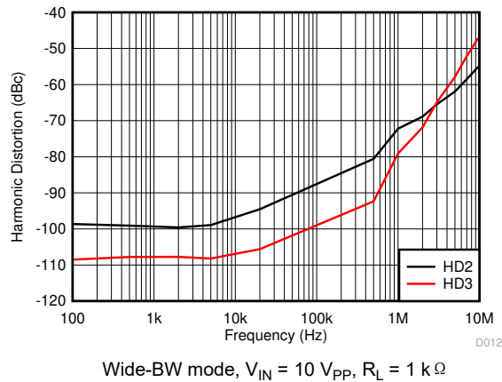
图 6-29. Harmonic Distortion vs Frequency
