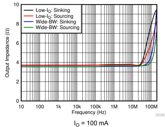
图 6-40. Output Impedance vs Frequency
