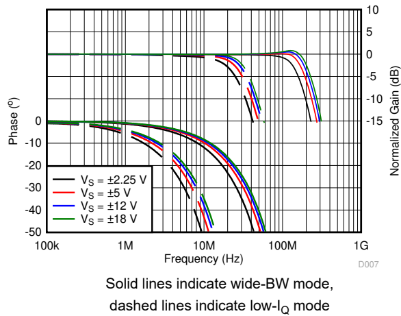
图 6-25. Gain and Phase vs Frequency and Power-Supply Voltage
