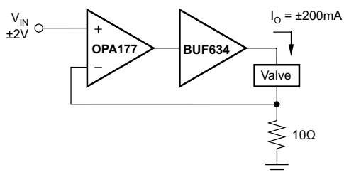
图 8-4. Current-Output Valve Driver
