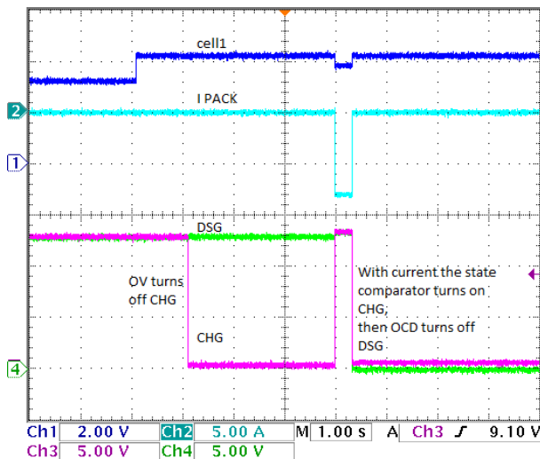
图 10-12. OV and OCD2 Faults Protection
