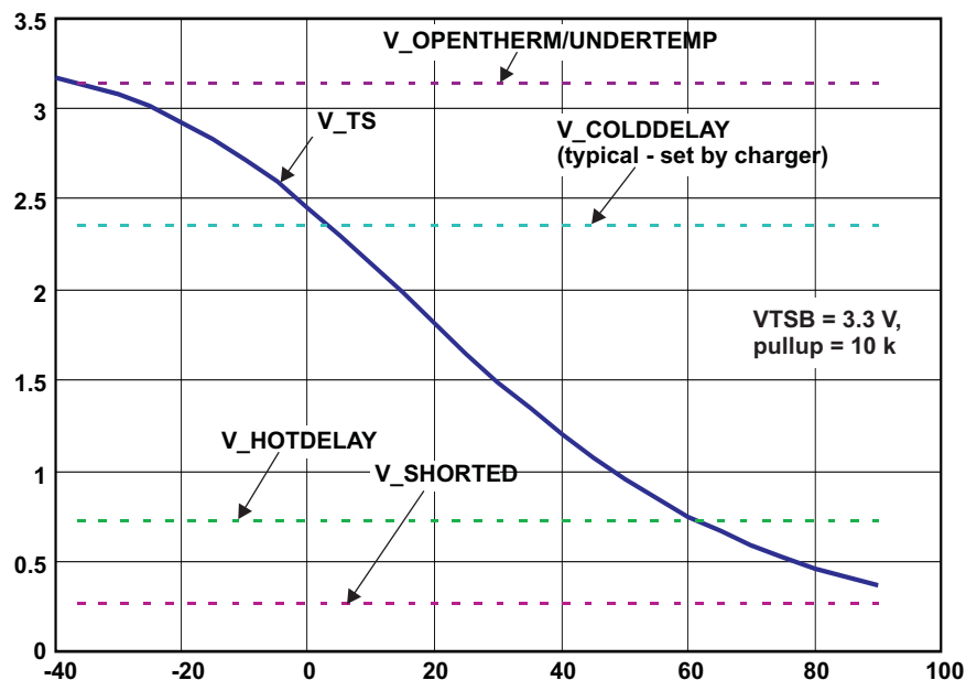
图 13. Typical Thermistor Response and Protection Thresholds ( V_{TSB} = 3.3\text{ V} , Pullup = 10\text{ k}\Omega )
