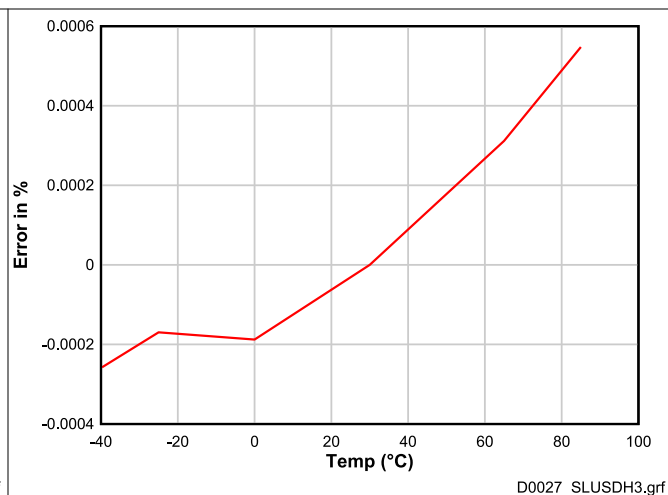
图 7-23. Coulomb Counter Gain Error vs. Temperature
