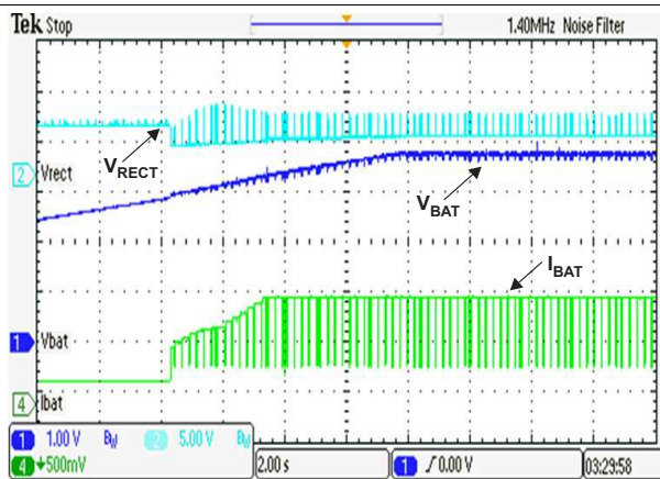
Figure 15. Precharge to Fast-Charge Transition
