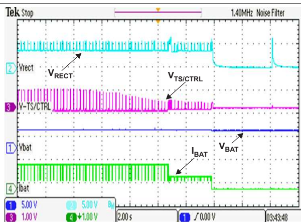
Figure 17. JEITA Functionality (Falling Temp) - bq51050B/bq51051B
