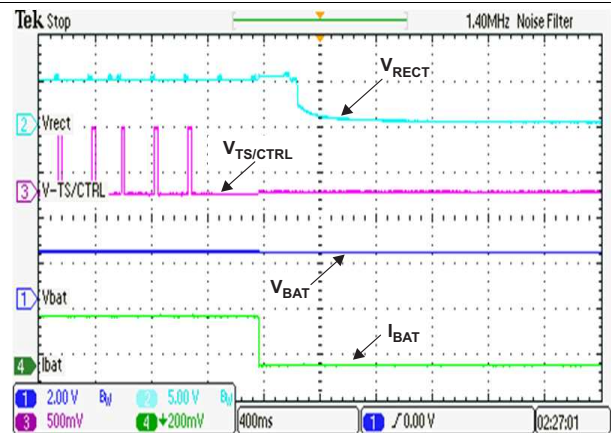
Figure 14. TS Ground Fault
