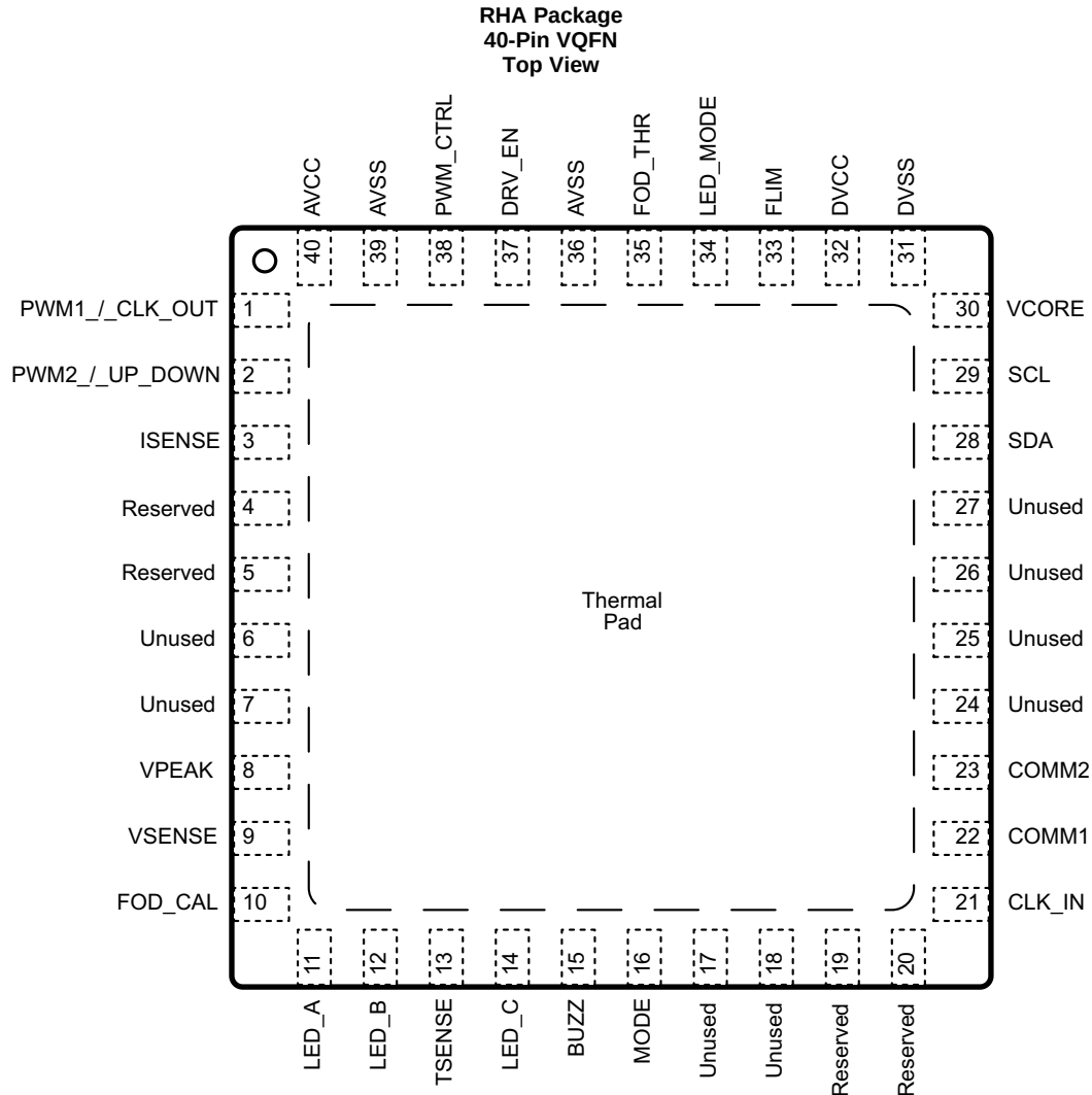
Pin Functions
