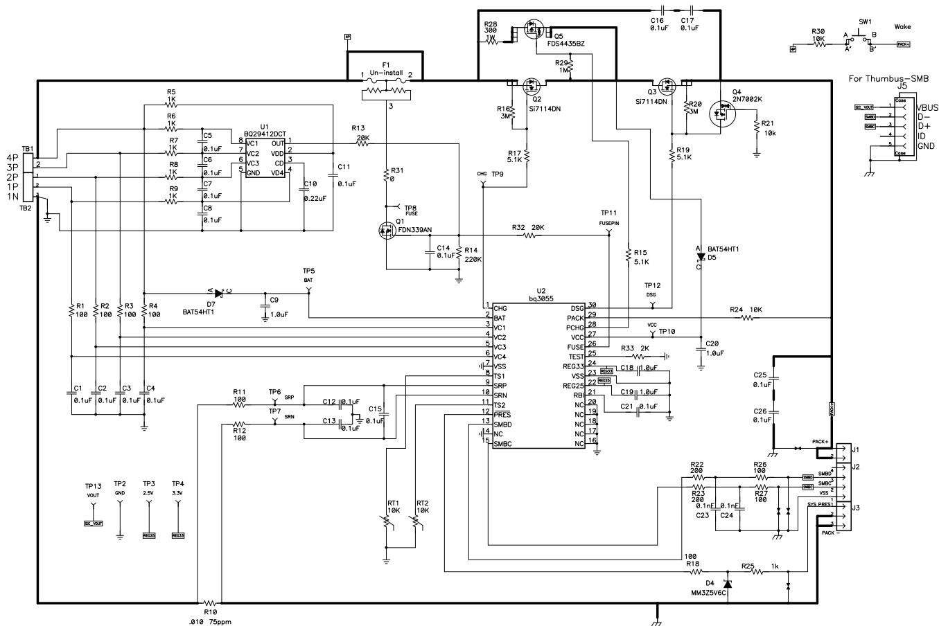
Figure 6. Application Schematic
