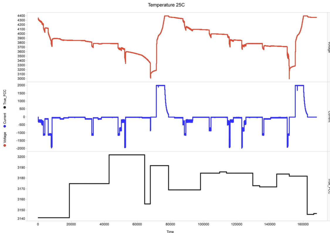
Figure 7-3. Full Charge Capacity Tracking (X-Axis Is Seconds)
