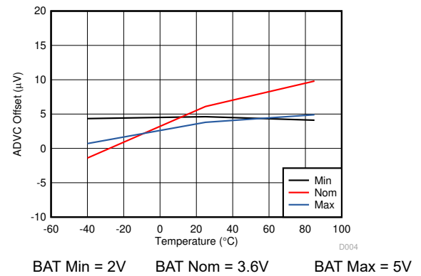
Figure 5-6. ADVC Offset Voltage Versus Battery and Temperature
