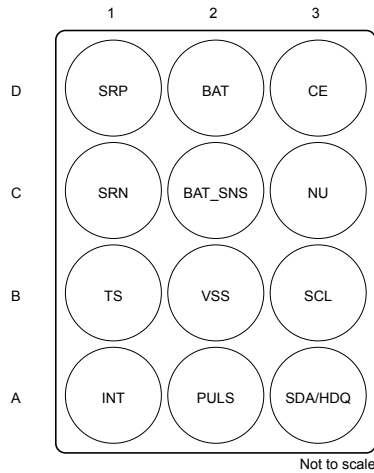
Figure 4-1. Pin Diagram
