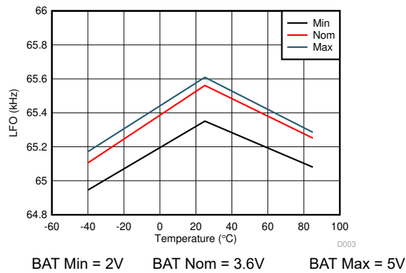
Figure 5-5. LFO Frequency Versus Battery and Temperature
