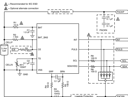
Simplified Schematic
