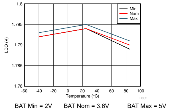
Figure 5-4. LDO Voltage Versus Battery and Temperature
