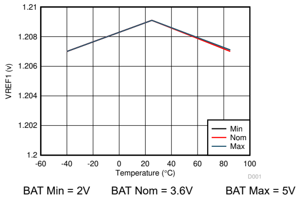
Figure 5-3. REF1 Voltage Versus Battery and Temperature
