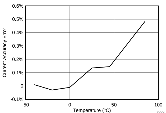
Figure 3. Current Accuracy Error vs. Temperature
