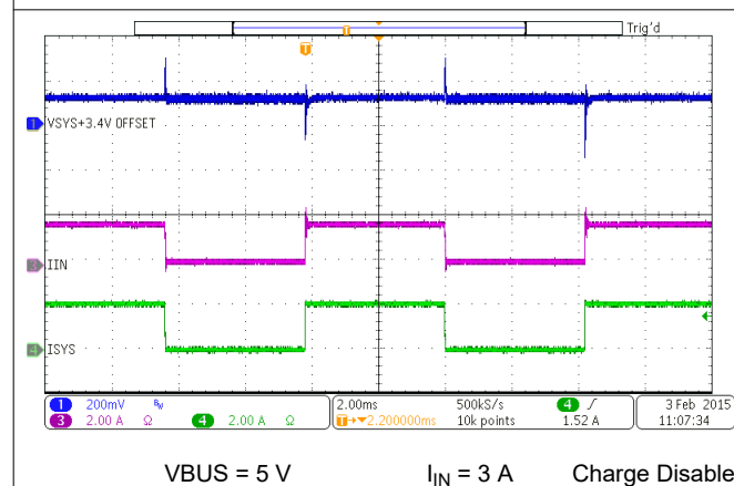
图 9-6. Input Current DPM Response without Battery
