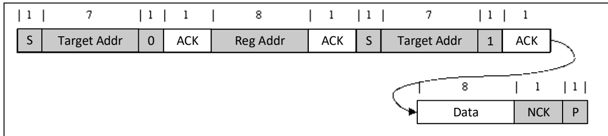
图 8-14. Single Read
