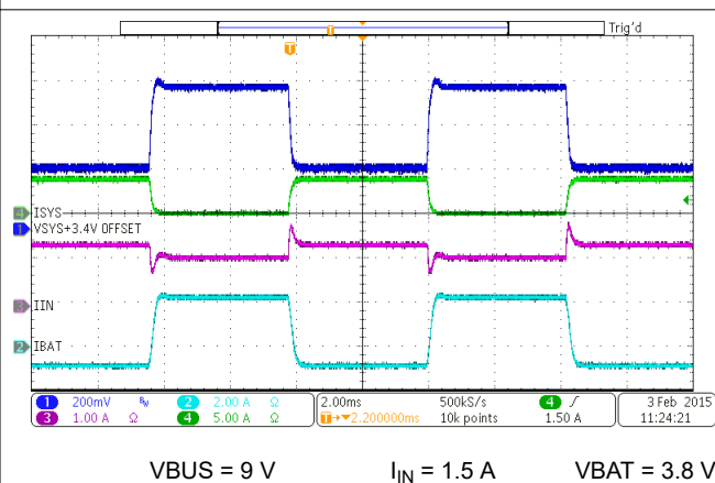
图 9-5. Charge Disable
