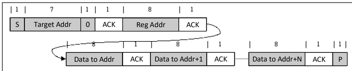
图 8-15. Multi-Write
