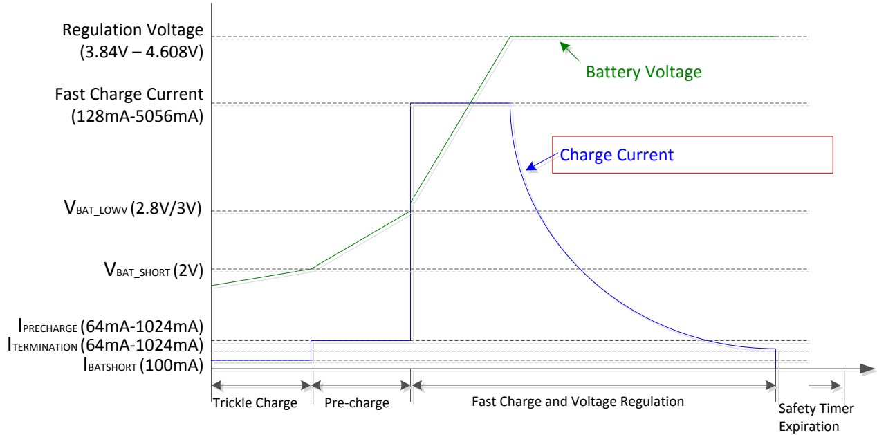
图 8-5. Battery Charging Profile
