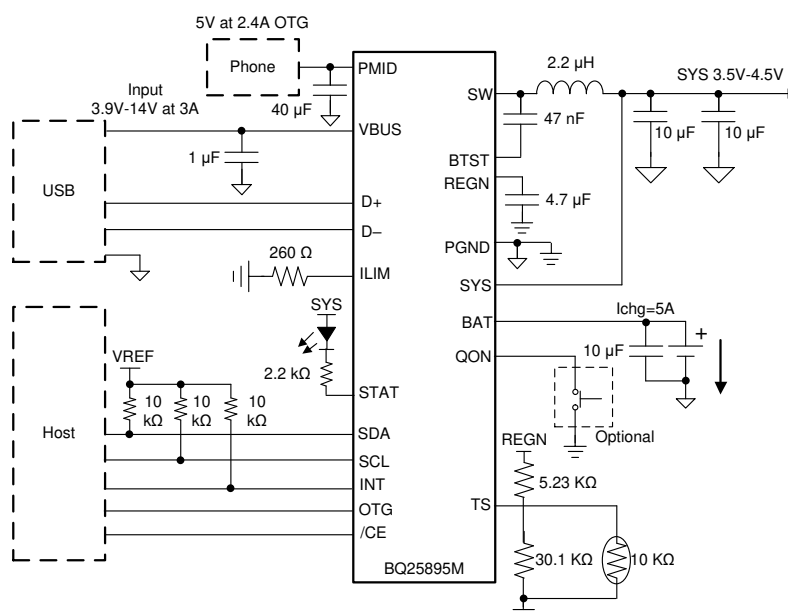
图 9-1. BQ25895M with D+/D- Interface and 2.4 A Boost Mode Output
