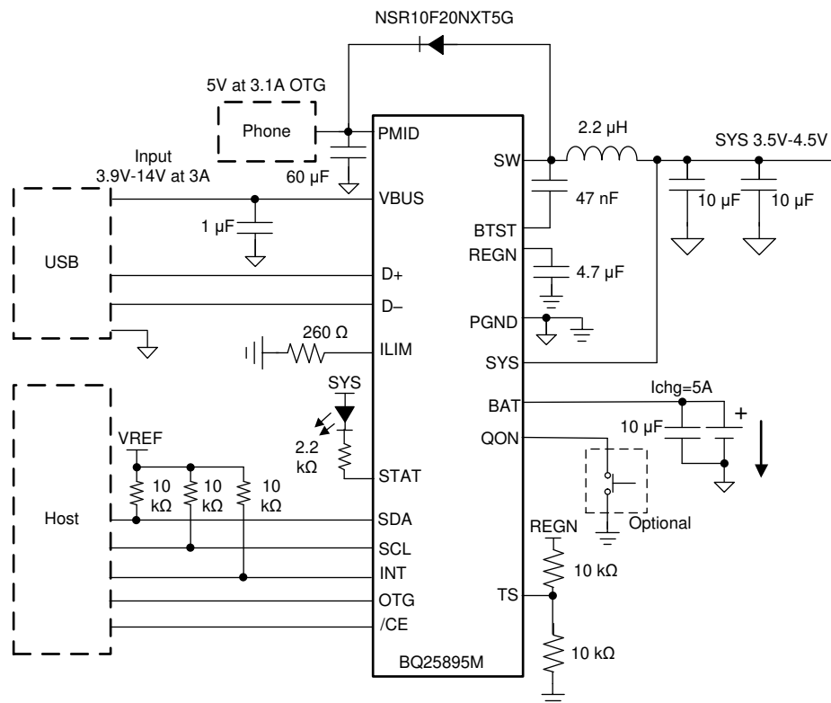
图 9-12. BQ25895M with D+/D- Interface, 3.1 A Boost Mode Output, and No Thermistor Connections
