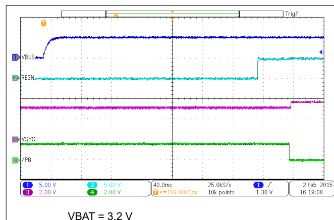
图 9-2. Power Up with Charge Disabled
