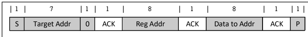
图 8-13. Single Write
