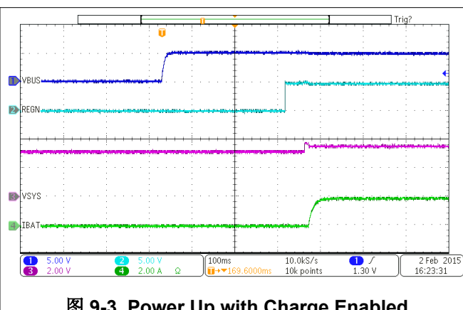
图 9-3. Power Up with Charge Enabled
