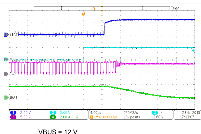
图 9-5. Charge Disable
