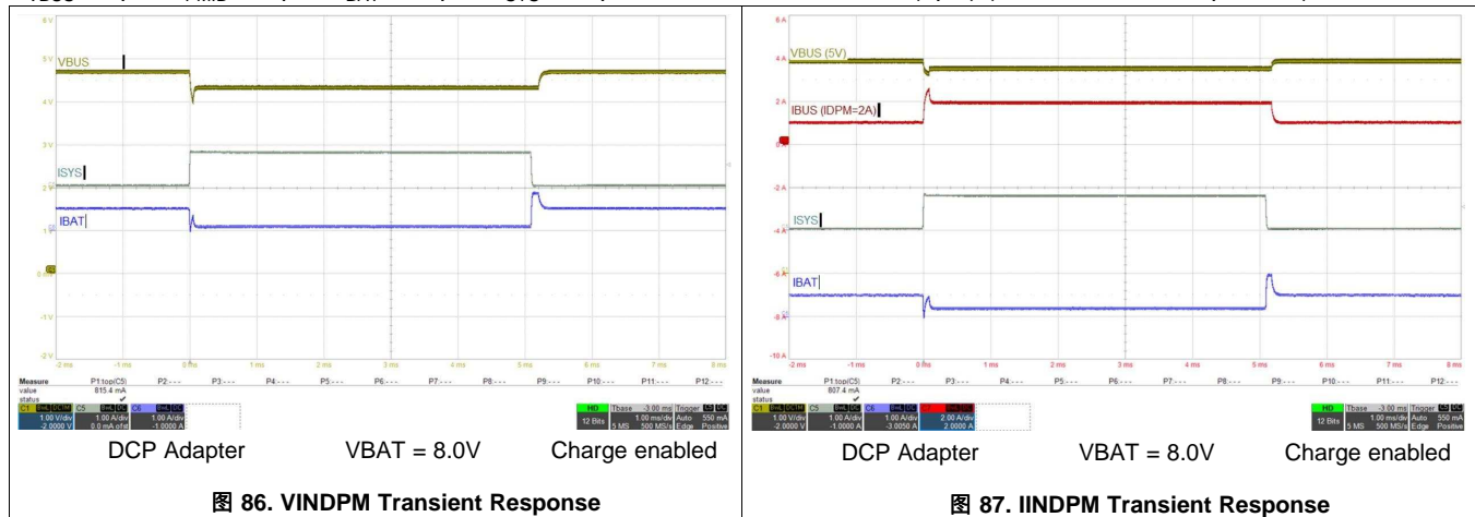
图 86. VINDPM Transient Response
