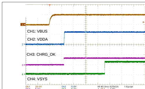
图 42. Power Up from 20 V
