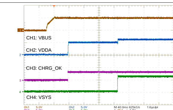
图 43. Power Up from 5 V
