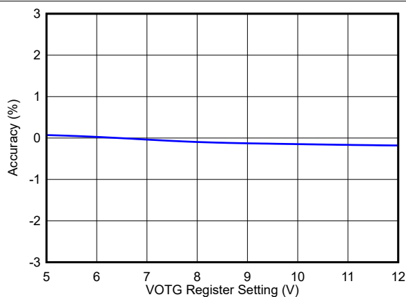
图 7-19. OTG Voltage Regulation (VOTG) Accuracy
