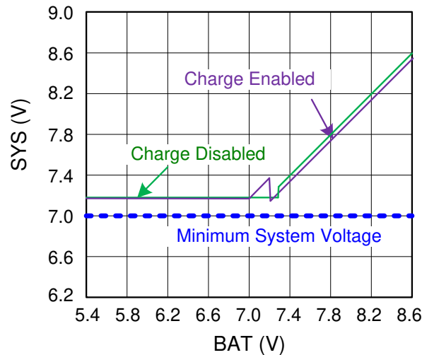
图 8-7. Typical System Voltage vs Battery Voltage for a 2S Battery Configuration
