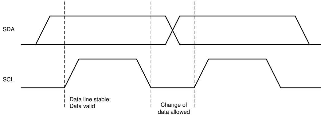
图 8-15. Bit Transfers on the I 2 C Bus
