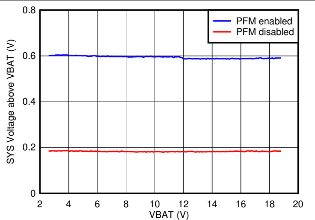
图 7-20. Offset Voltage of SYS Regulation above VBAT
