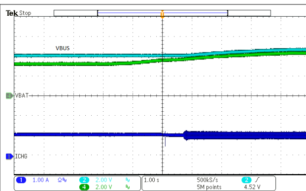
图 10-21. VINDPM Tracking Battery Voltage
