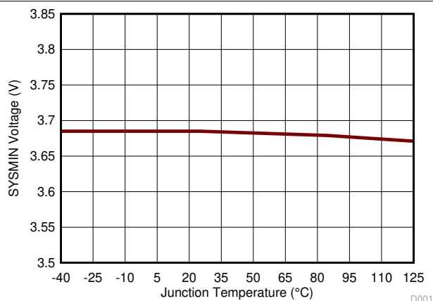
图 8-5. SYSMIN Voltage vs. Junction Temperature
