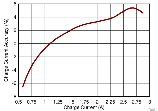
图 8-4. Charge Current Accuracy
