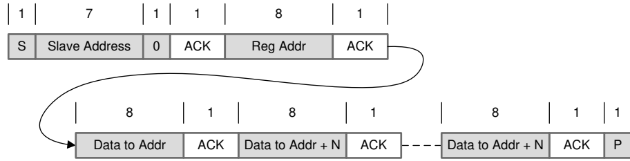
图 9-18. Multi-Write
