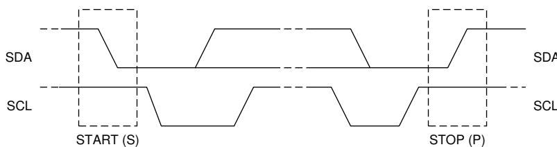
图 9-13. TS START and STOP Conditions
