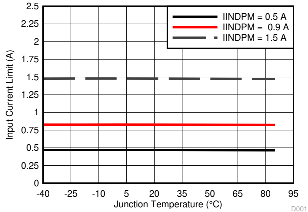
图 8-7. Input Current Limit vs. Junction Temperature
