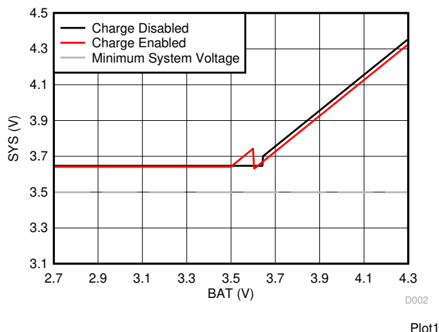
图 9-7. System Voltage vs Battery Voltage
