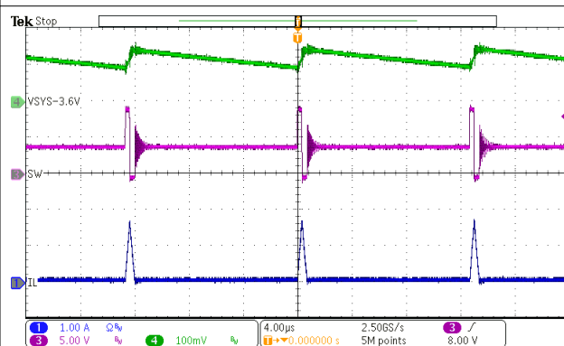
图 10-3. Power-Up with Charge Enabled
