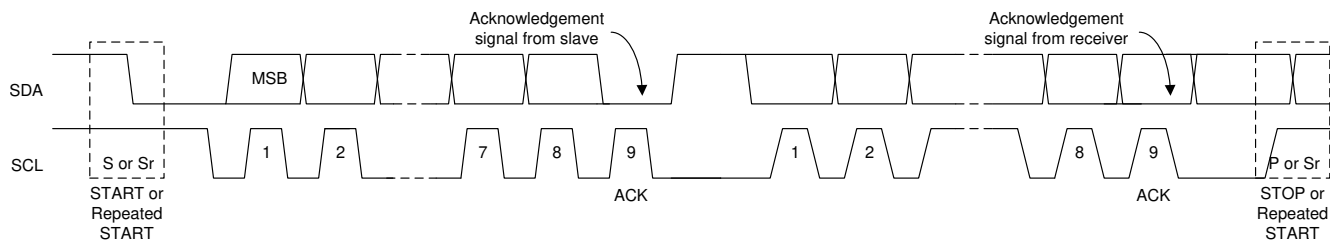
图 9-14. Data Transfer on the I²C Bus
