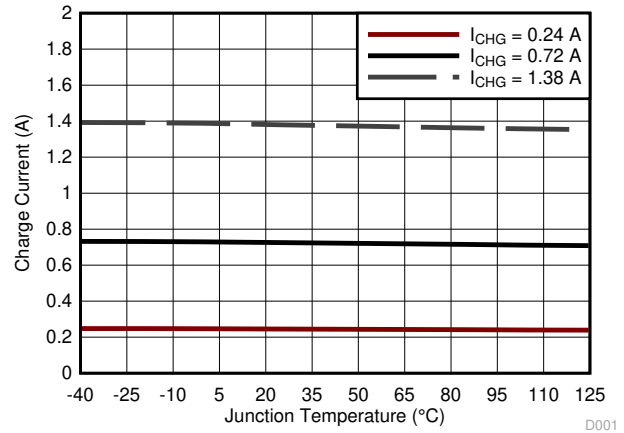
图 8-8. Charge Current vs. Junction Temperature
