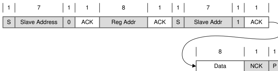
图 9-17. Single Read
