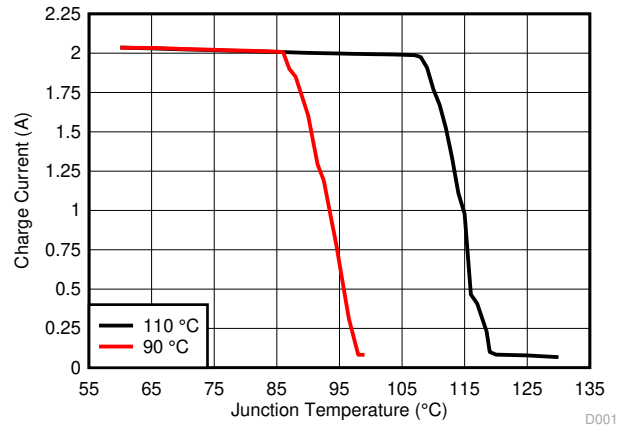
图 8-9. Charge Current vs. Junction Temperature
