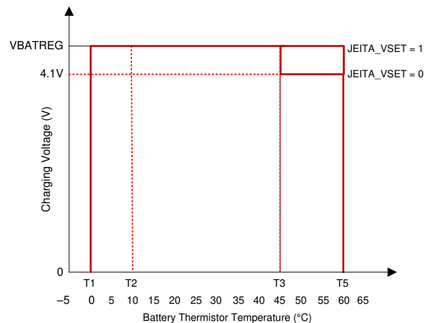
图 9-4. JEITA Profile: Charging Voltage
