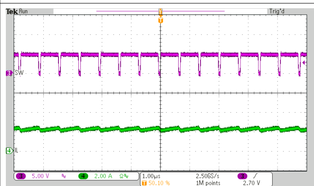
图 10-5. PFM Switching in Buck Mode
