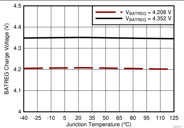
图 8-6. BATREG Charge Voltage vs. Junction Temperature
