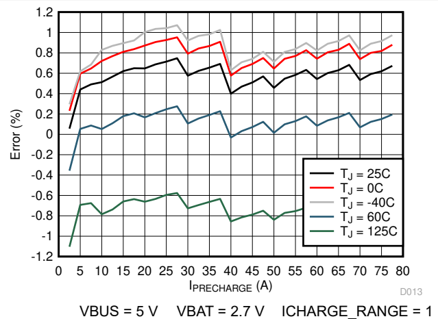
图 8-4. Pre-Charge Current Accuracy vs. IPRECHARGE Setting (ICHARGE_RANGE = 1)
