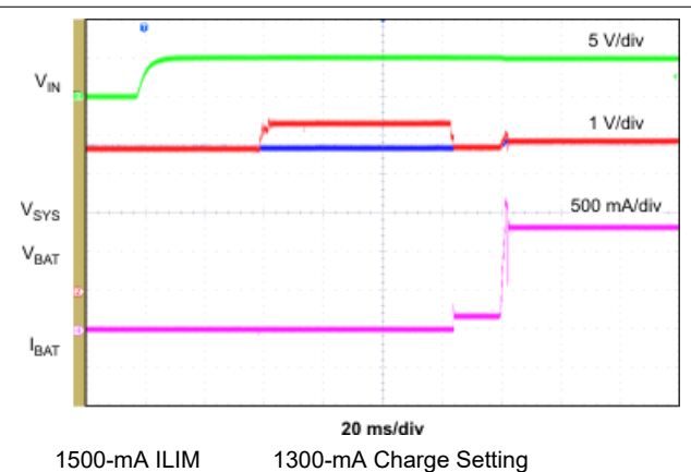
图 9-4. IN Plug-in with Battery Connected
