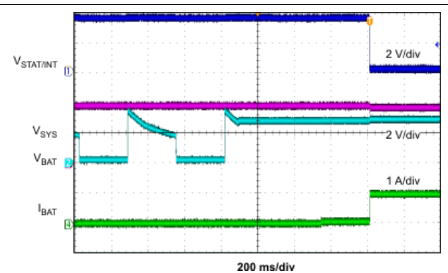
图 9-4. IN Plug-in with Battery Connected
