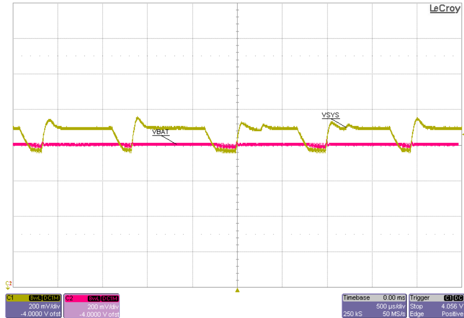
图 8-7. V(SYS) When Reverse Boost Prevention Circuit is Active
