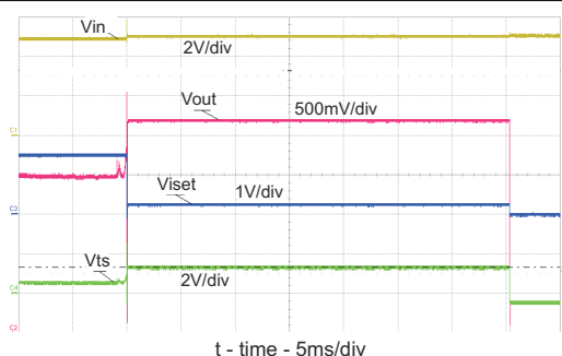
图 9-10. Battery Removal - GND Removed 1st, 42 \Omega Load
