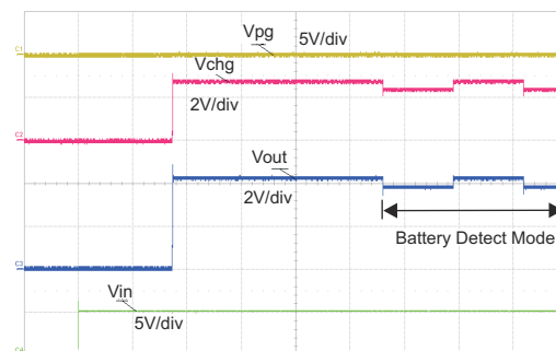
图 9-9. Hot Plug Source w/No Battery - Battery Detection
