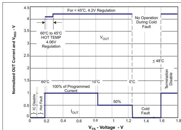
图 8-4. Operation Over TS Bias Voltage (BQ24040)
