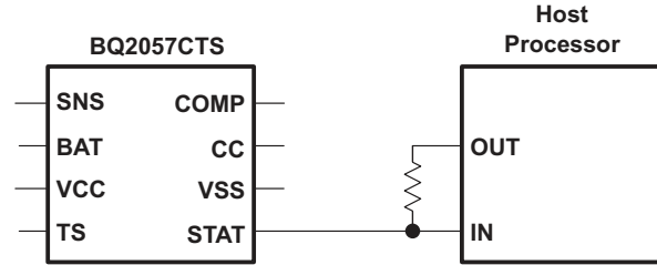
图 10-11. Interfacing the BQ2057 to a Host Processor
