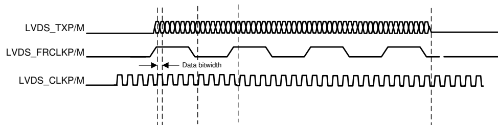
图 8-7. LVDS Interface Lane Configuration And Relative Timings
