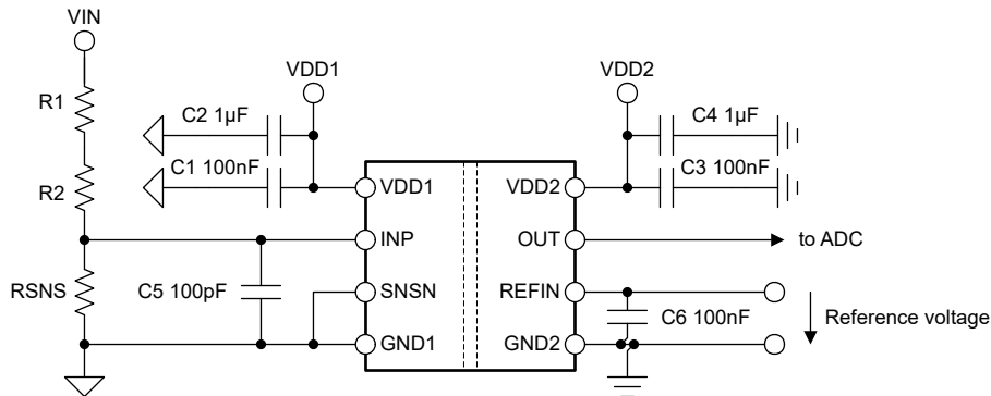
图 8-5. AMC0x30S 去耦
