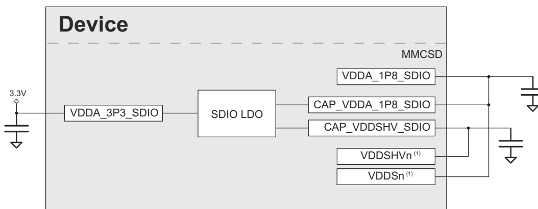
图 8-11. VDDSHV6 or VDDSHV7 Used as the MMCSDB Supply for Fixed 3.3V IO
