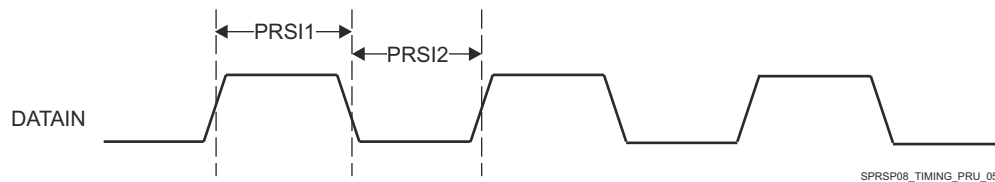
图 6-98. PRU_ICSSG PRU Shift In Timing
