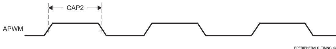
图 6-42. eCAP Switching Characteristics
