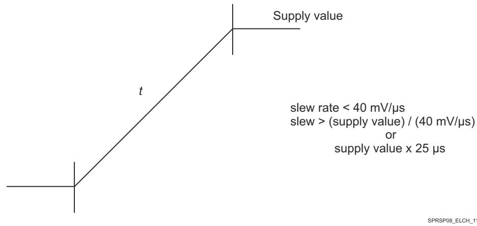
图 6-3. VDDA_1P8_SERDES0 Supply Slew and Slew Rate
