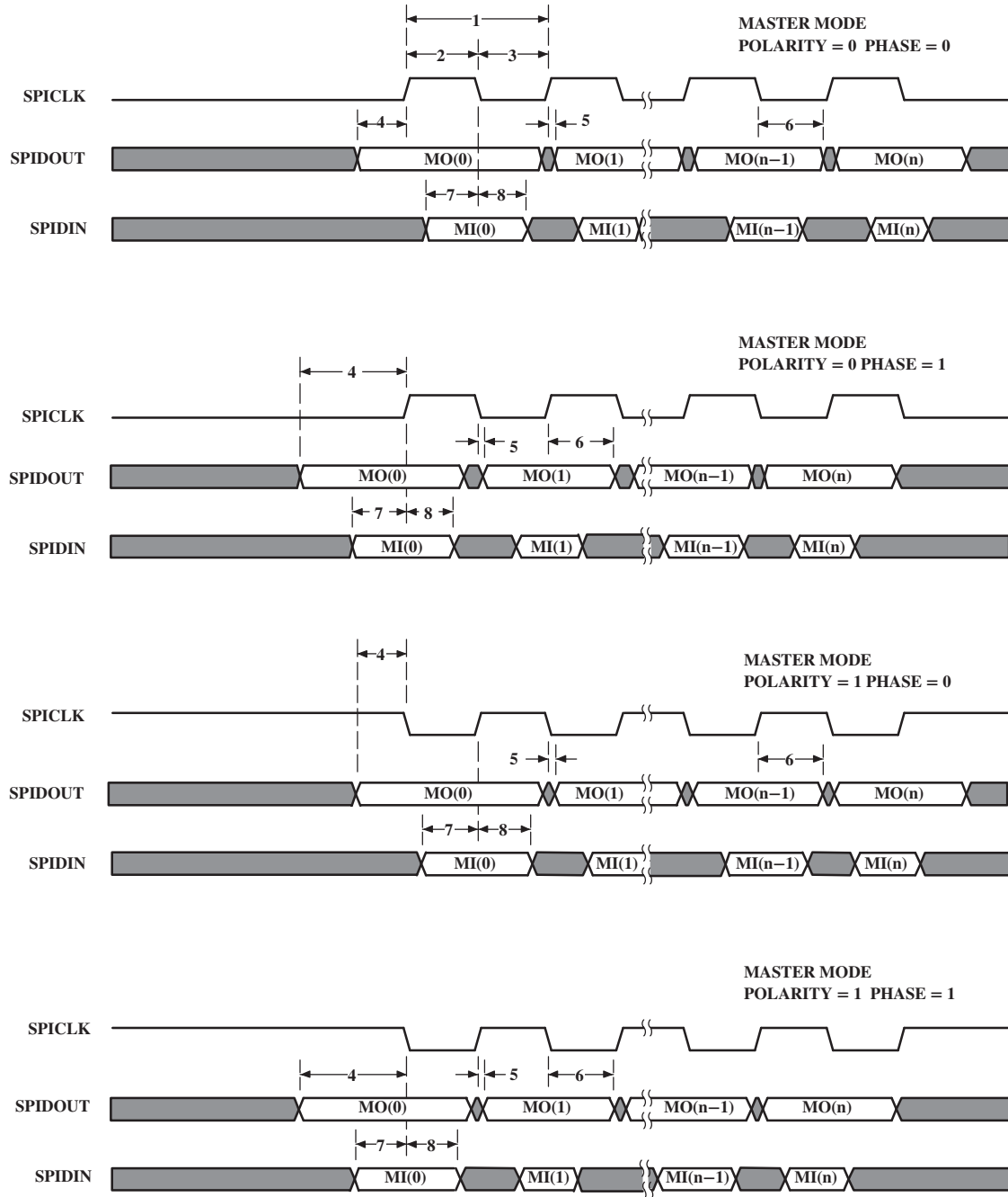
图 10-33. SPI Master Mode Timing Diagrams — Base Timings for 3-Pin Mode
