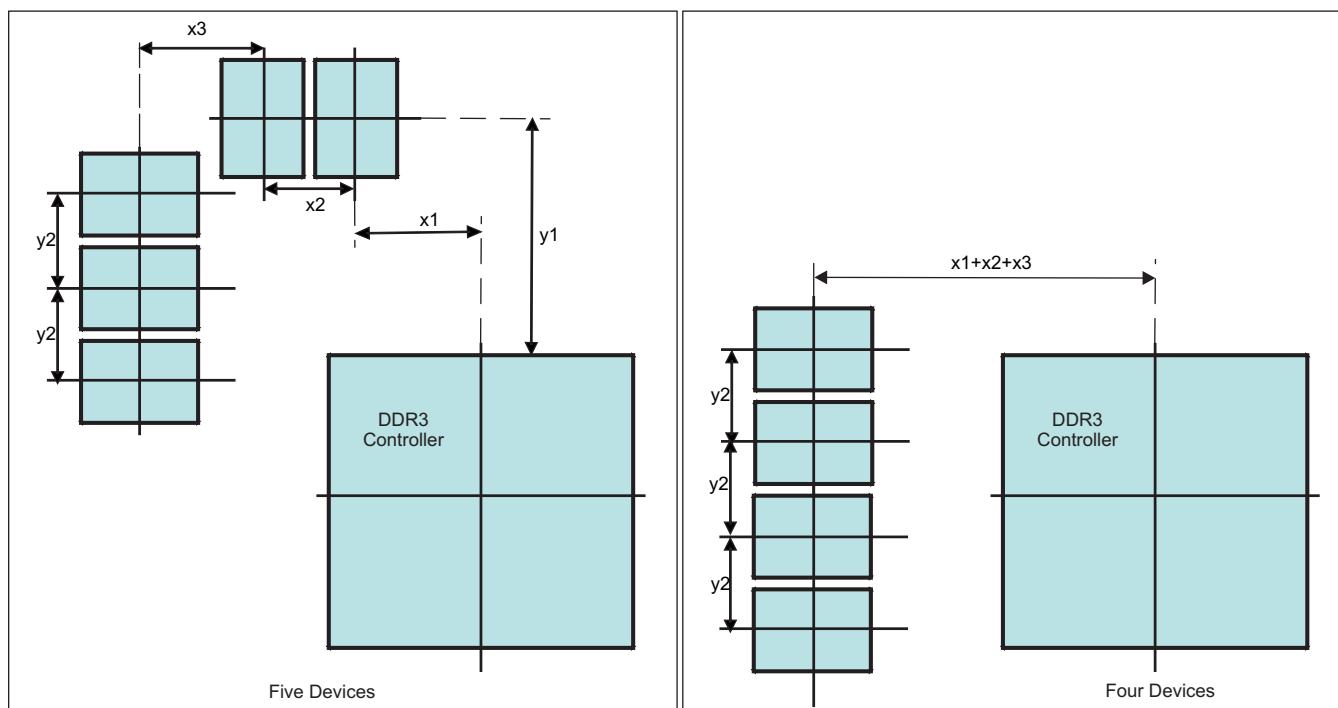
Figure 8-4. Placement Specifications
