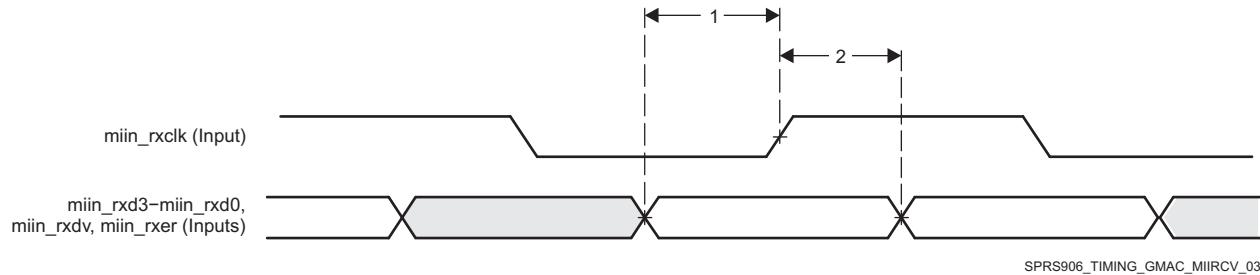
Figure 7-54. GMAC Receive Interface Timing MII n operation
