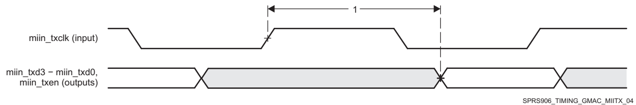
Figure 7-55. GMAC Transmit Interface Timing MII n operation
