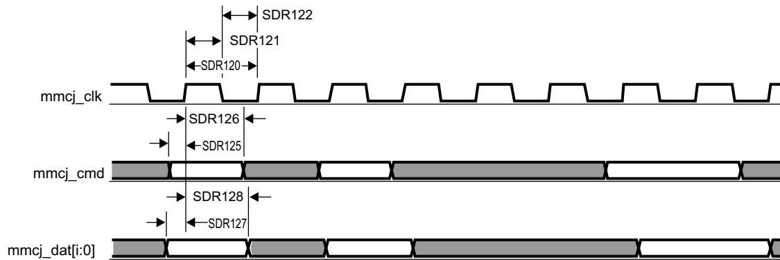
图 5-98. MMC/SD/SDIOj in - SDR12 - Receiver Mode
