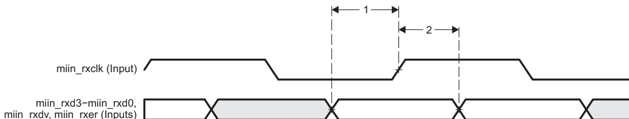
图 5-66. GMAC Receive Interface Timing MII operation
