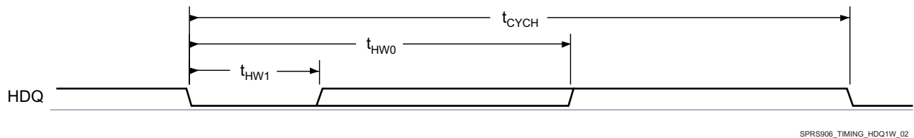
图 5-39. Device HDQ Interface Bit Read Timing (Data)
