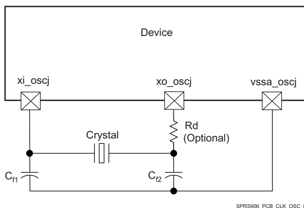
图 7-31. Grounding Scheme for High-Frequency Clock
