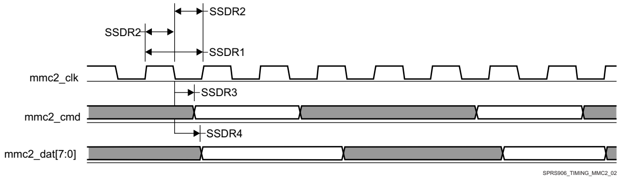
图 5-88. MMC/SD/SDIO in - Standard JC64 - Transmitter Mode
