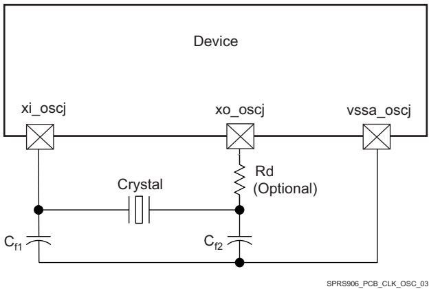
图 7-31. Grounding Scheme for High-Frequency Clock
