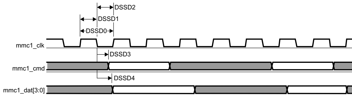
图 5-74. MMC/SD/SDIO in - Default Speed - Transmitter Mode
