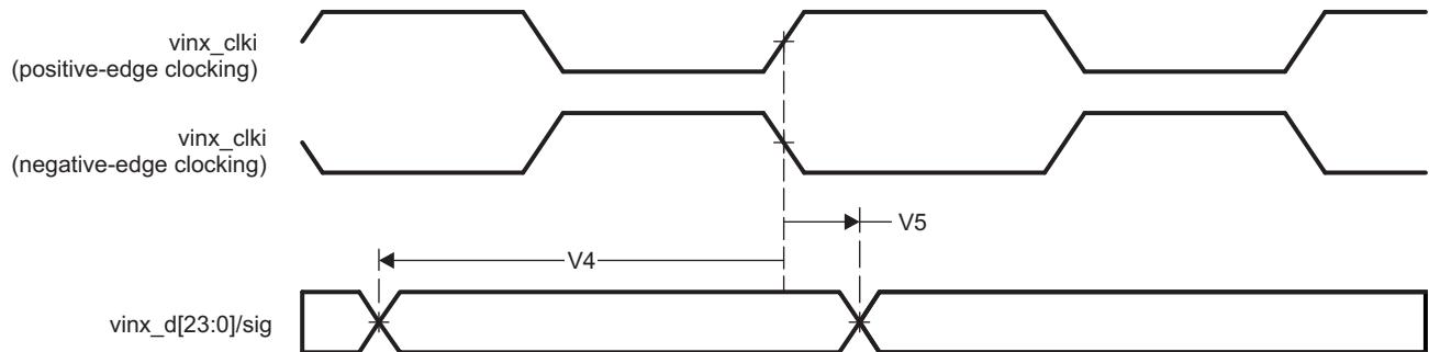
图 5-18. Video Input Ports timings
