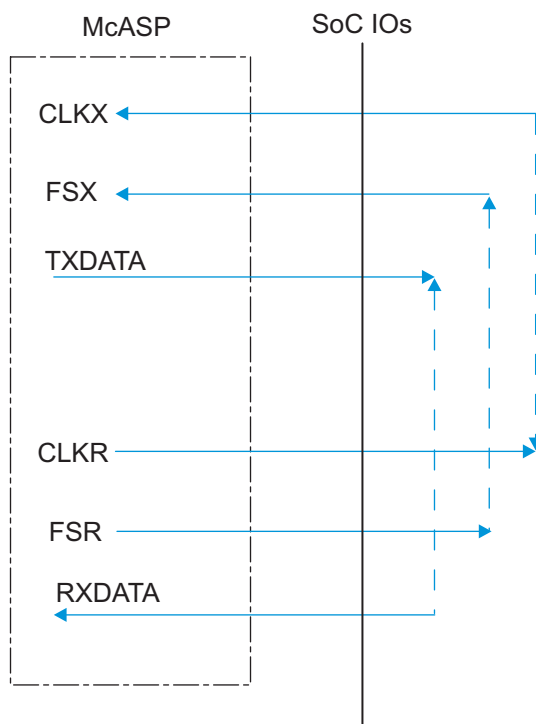
图 5-58. McASP1-8 CIOFIO – ASYNC Mode
