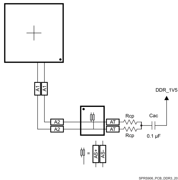
图 7-20. CK Routing for One DDR3 Device
