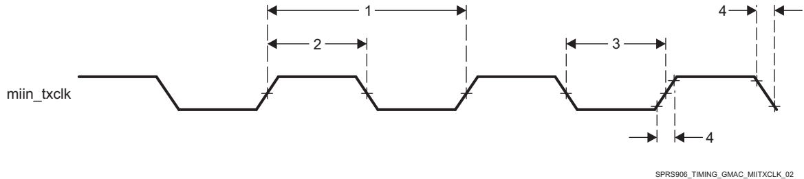
图 5-65. Clock Timing (GMAC Transmit) - MII operation
