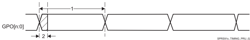
图 5-105. PRU-ICSS PRU Direct Output Timing
