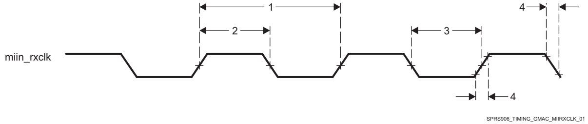
图 5-64. Clock Timing (GMAC Receive) - MII operation
