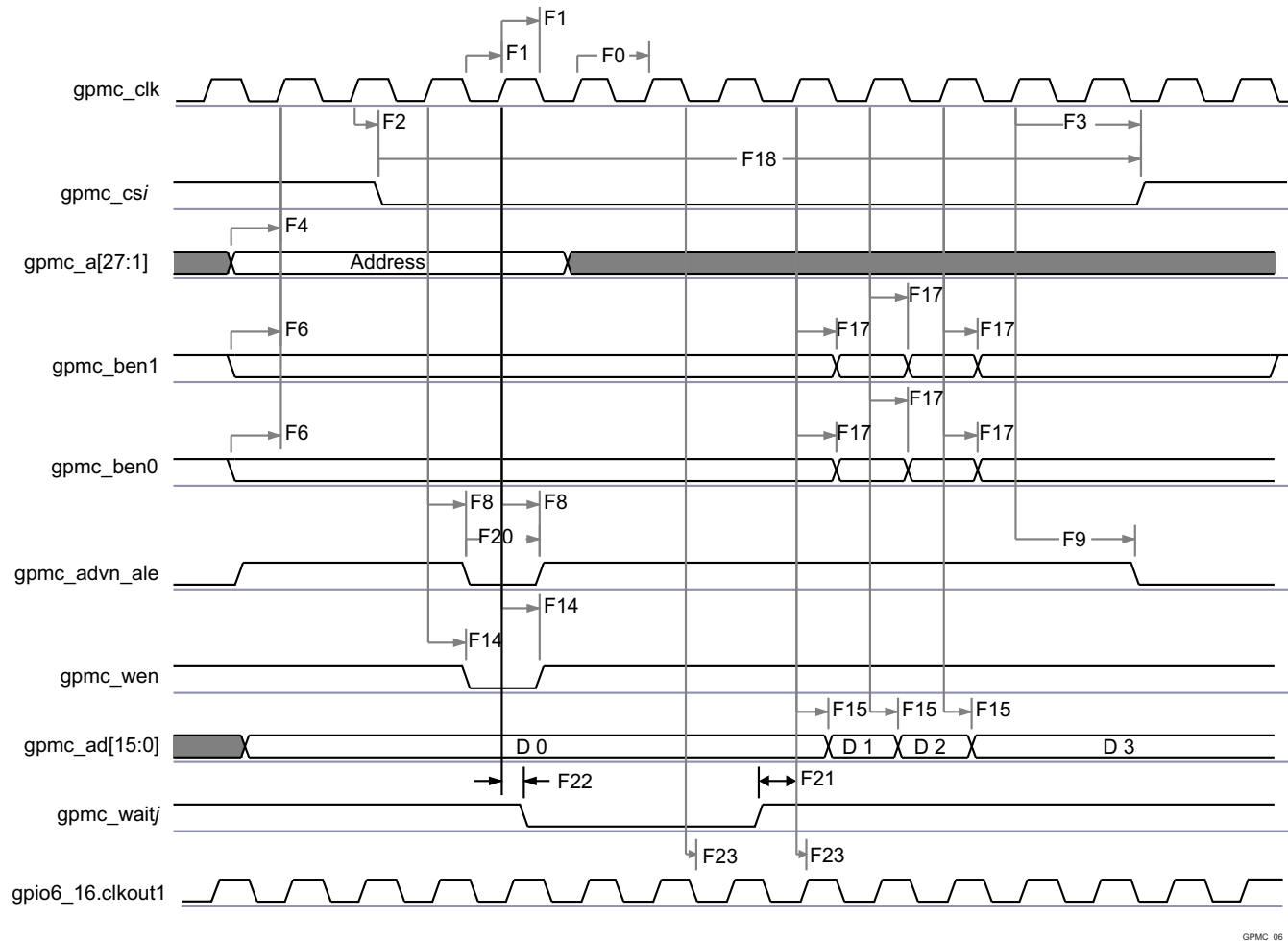
图 5-25. GPMC / Nonmultiplexed 16bits NOR Flash - Synchronous Burst Write 4x16bits - (GpmcFCLKDivider = 0) (1)(2)
