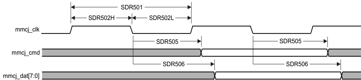
图 5-103. MMC/SD/SDIOj in - High Speed SDR50 - Transmitter Mode
