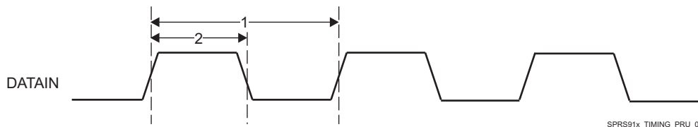
图 5-108. PRU-ICSS PRU Shift In Timing
