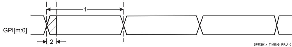
图 5-104. PRU-ICSS PRU Direct Input Timing
