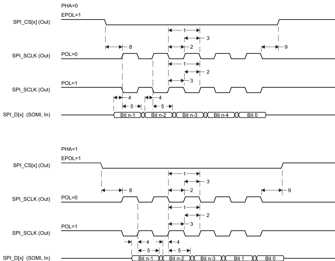
图 5-108. SPI Master Mode Receive Timing
