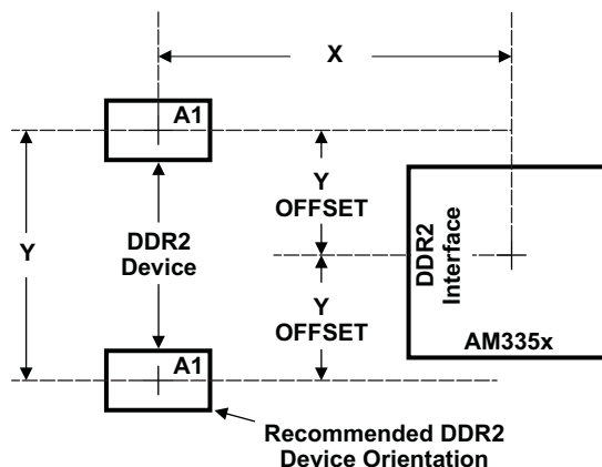
图 7-41. AM3358-EP Device and DDR2 Device Placement
