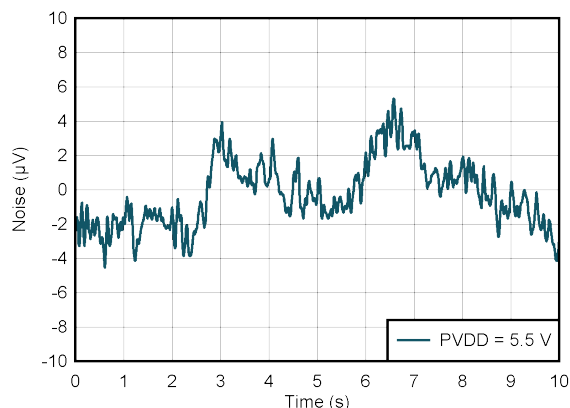
DAC 处于中间码 PVDD = 5.5V
