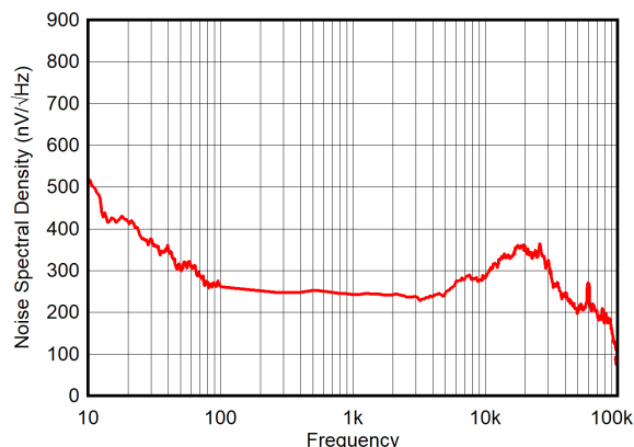
DAC 处于中间码 PVDD = 5.5V
