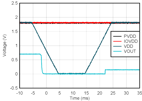
图 6-31. DAC VDD Supply Collapse Response, RANGE = 0
