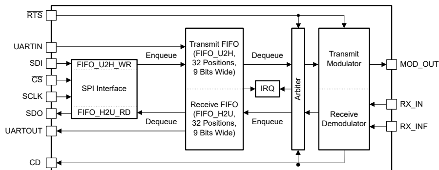
图 7-17. HART Architecture
