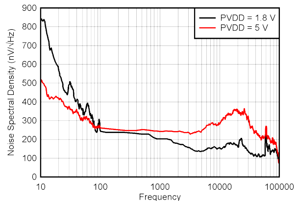
图 6-20. DAC Output Noise Density vs Frequency
