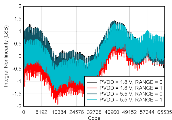
图 6-5. DAC INL vs Digital Input Code
