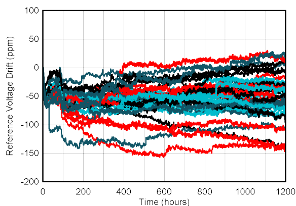
图 6-46. Reference Voltage Long-Term Stability
