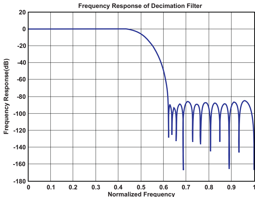
Figure 9-2. Decimation Filter Frequency Response (from 0 to F_{\text{ADCCLK}}/2 )
