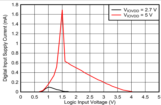
图 6-50. Supply Current vs Input Voltage
