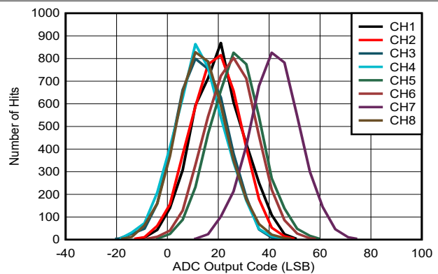
图 5-35. V_{IN} = 1mV 时的直流代码直方图, 宽带宽, RANGE = \pm 5V
