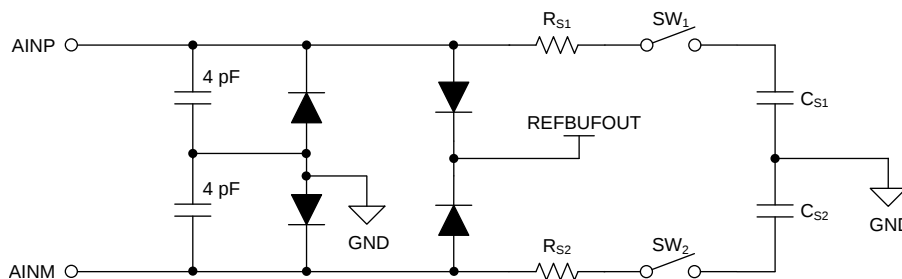
Figure 37. Input Sampling Stage Equivalent Circuit
