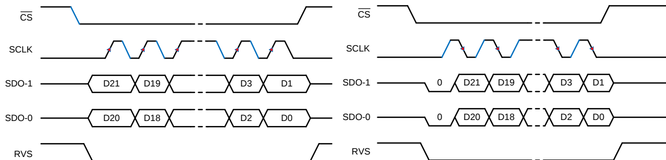
Figure 62. SPI-00-D Protocol
