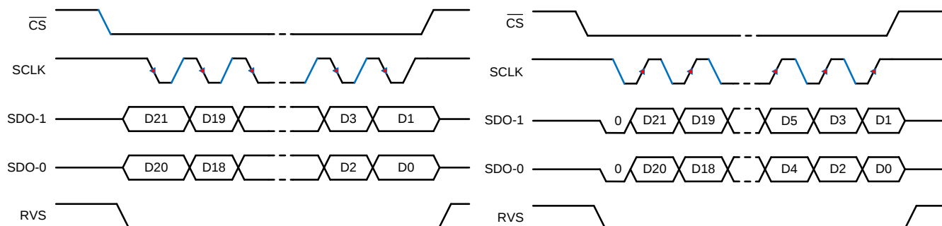
Figure 64. SPI-10-D Protocol
