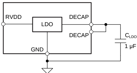
Figure 30. Internal LDO Connections
