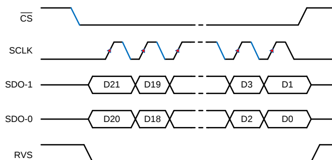
Figure 60. SPI-00-D Protocol
