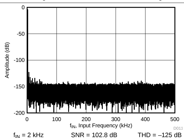
Figure 21. Typical FFT
