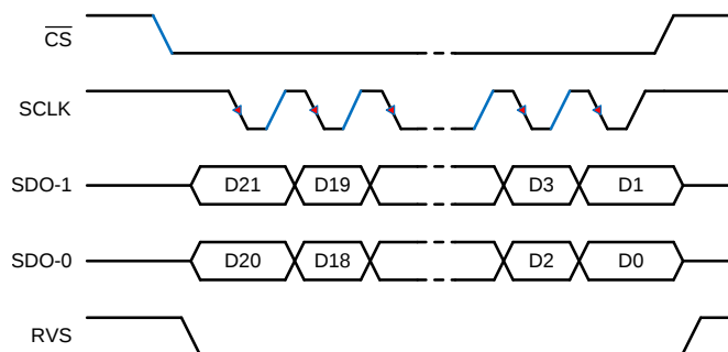
Figure 62. SPI-10-D Protocol
