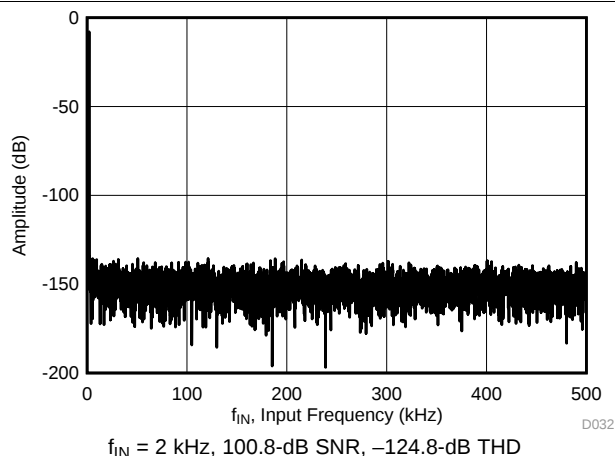
Figure 113. Noise-Performance FFT Plot: ADS8910B, Single-Ended Input
