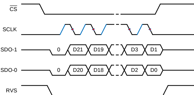
Figure 61. SPI-01-D Protocol
