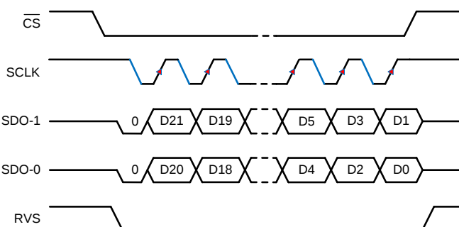
Figure 63. SPI-11-D Protocol
