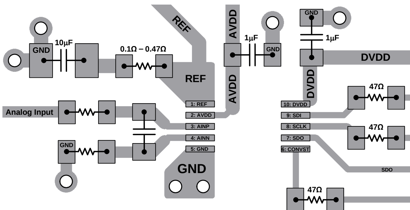
图 69. Recommended Layout
