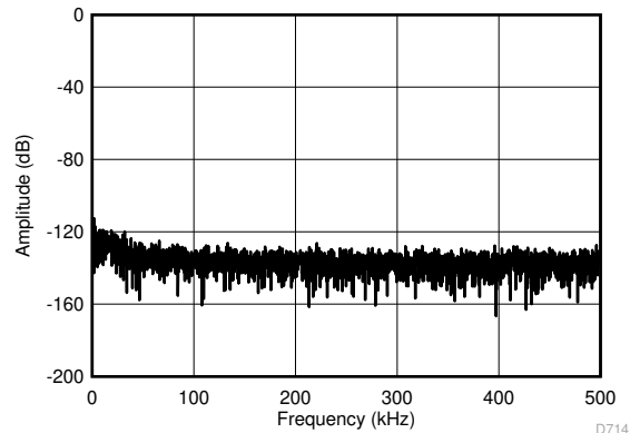
图 8-3. FFT Plot With a DC Common-Mode at 1 MSPS
