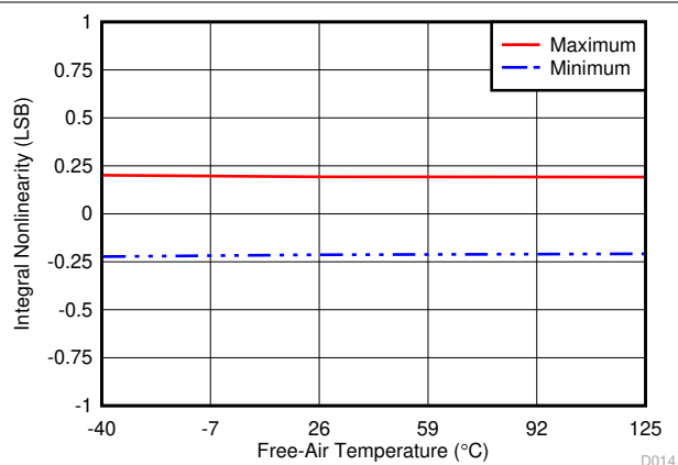
图 6-24. Typical INL for All Codes (All Bipolar Ranges)
