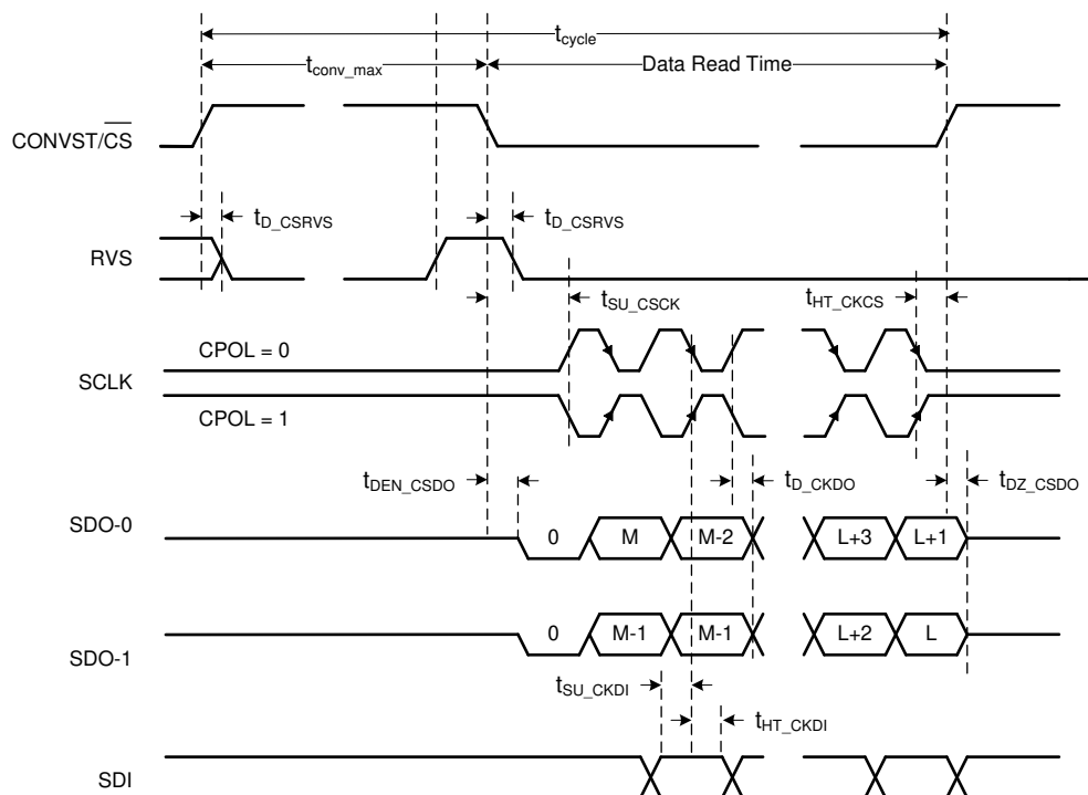
图 6-6. multiSPI Interface Timing Diagram for Dual SDO-x and CPOL = 1
