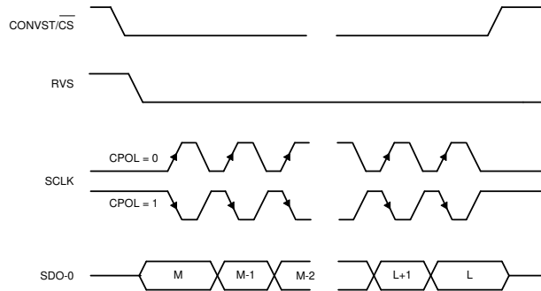
图 7-28. Standard SPI Timing Protocol (CPHA = 0, Single SDO-x)
