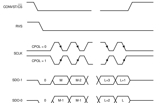
图 7-31. Standard SPI Timing Protocol (CPHA = 1, Dual SDO-x)
