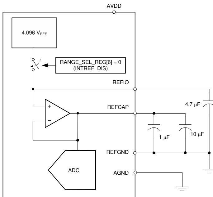
图 7-7. Device Connections for Using an Internal 4.096-V Reference
