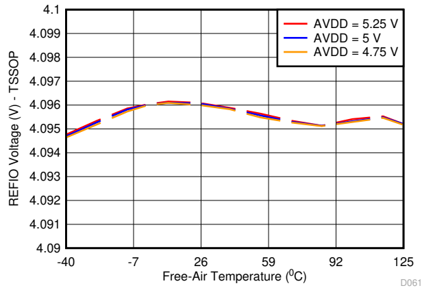
图 7-10. REFIO Voltage Variation Across AVDD and Temperature
