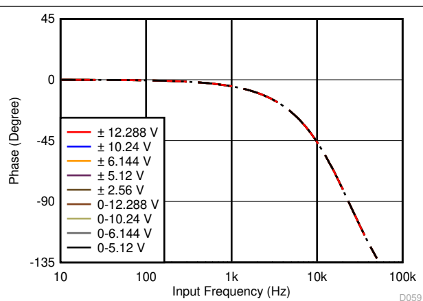
图 7-6. Second-Order LPF Phase Response
