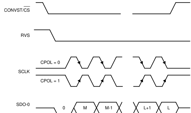
图 7-29. Standard SPI Timing Protocol (CPHA = 1, Single SDO-x)
