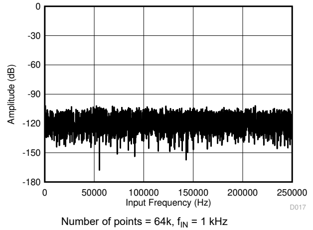
图 6-34. Typical FFT Plot (All Ranges) for the ADS8665
