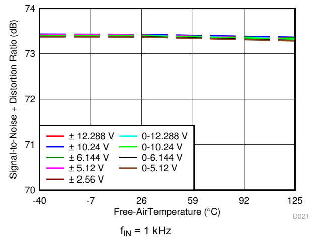
图 6-38. SINAD vs Temperature
