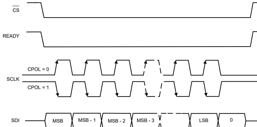
图 6-19. Standard SPI Timing Protocol (CPHA = 0)
