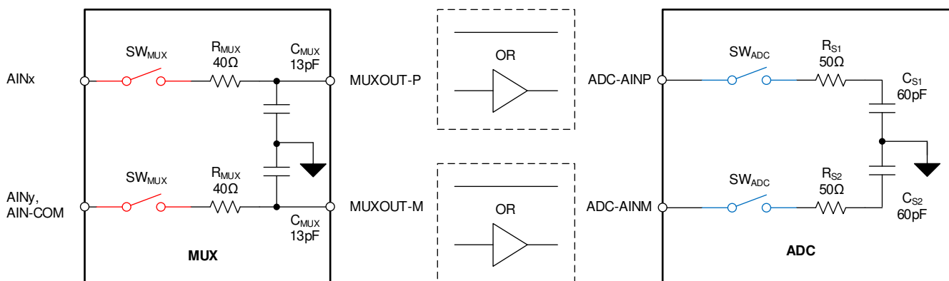
图 6-4. Synchronous and Timed Switching of the MUX and ADC Input Switches
