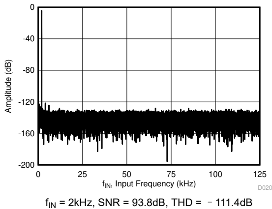
图 5-21. Typical FFT, ADS8166
