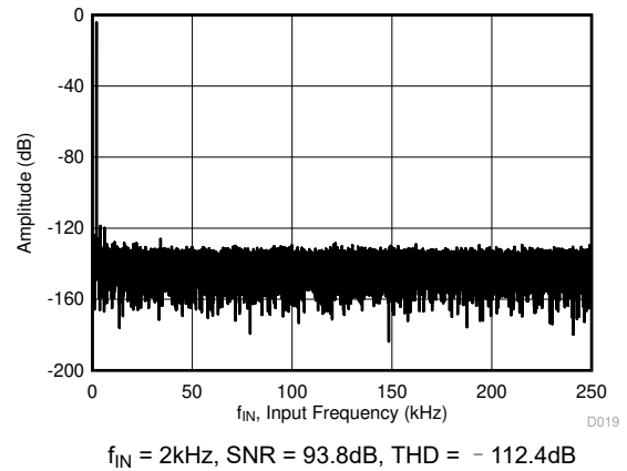
图 5-20. Typical FFT, ADS8167
