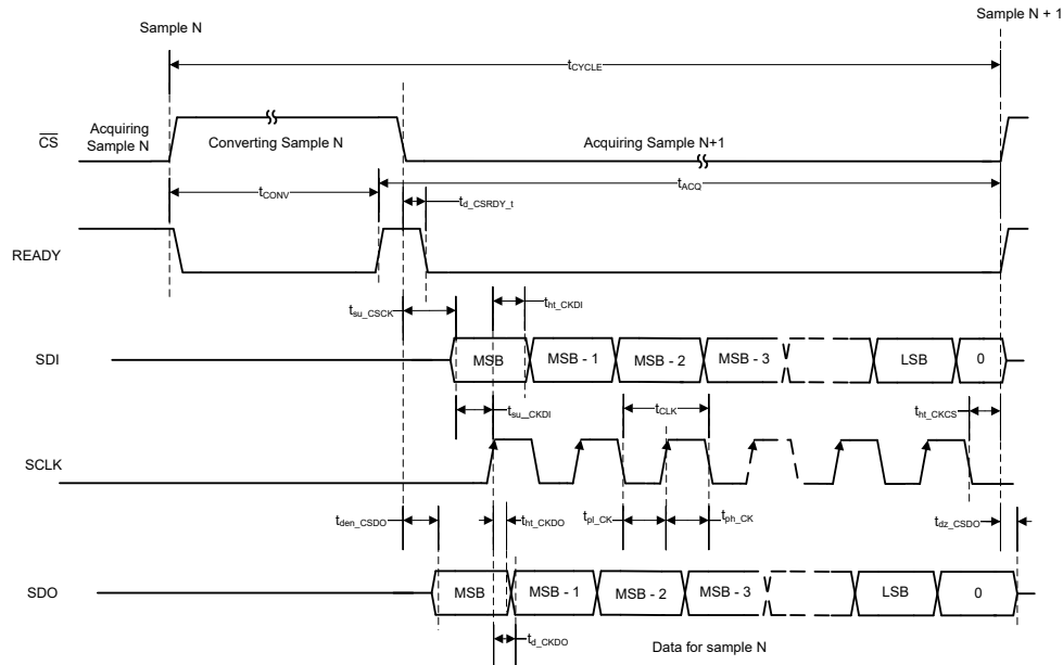
图 5-1. Conversion Cycle Timing: \overline{\text{CS}} = 1 Longer Than t_{\text{CONV}}
