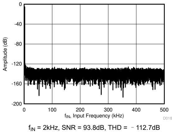
图 5-19. Typical FFT, ADS8168
