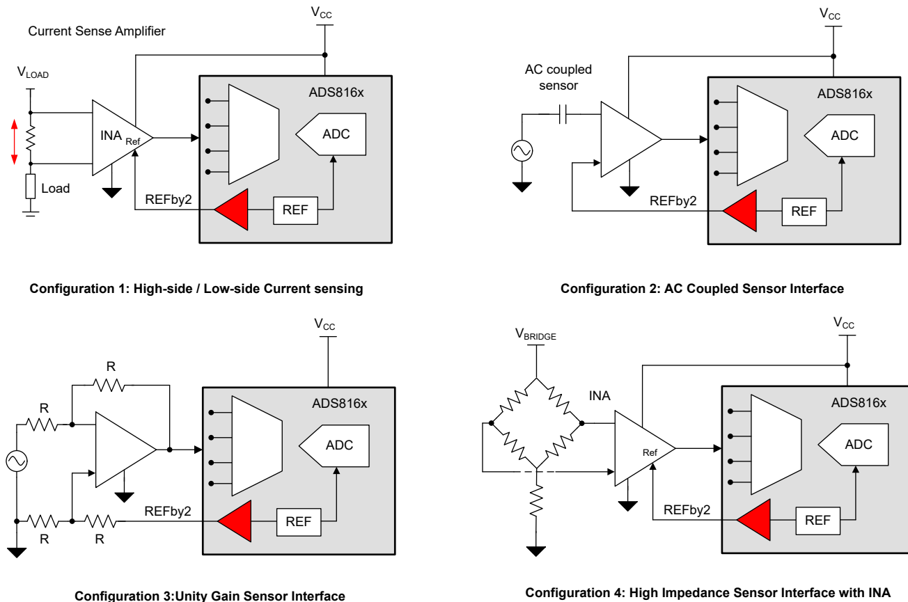
图 6-8. Signal Conditioning With the REFby2 Buffer
