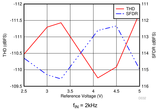
图 5-25. Distortion Performance vs Reference Voltage
