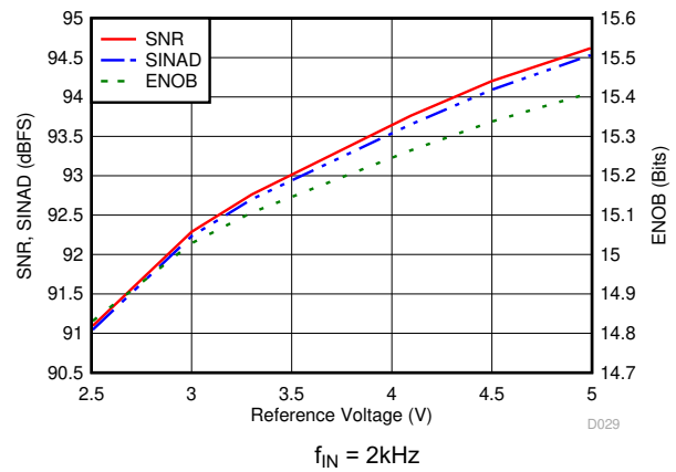
图 5-24. Noise Performance vs Reference Voltage
