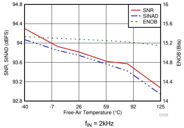
图 5-22. Noise Performance vs Temperature
