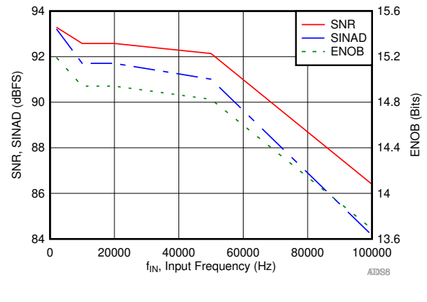
图 5-26. Noise Performance vs Input Frequency
