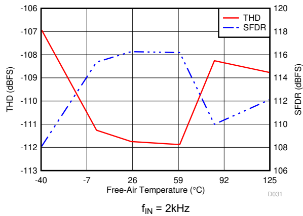
图 5-23. Distortion Performance vs Temperature
