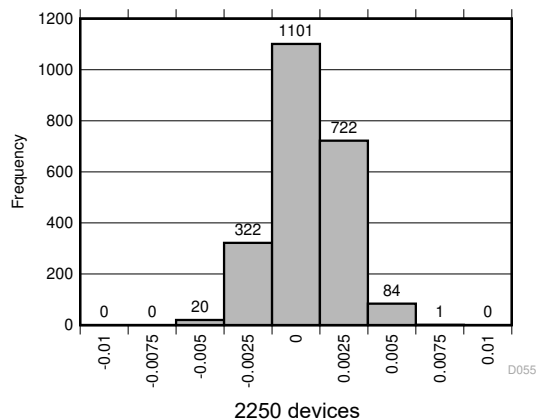
图 5-13. Typical Gain Error Distribution (%FSR)
