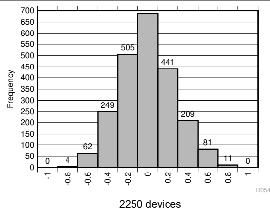
图 5-12. Typical Offset Distribution (LSB)
