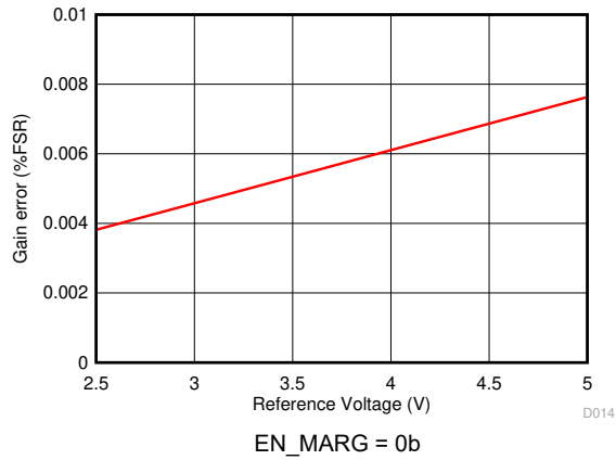
图 5-17. Gain Error (ADC + REFBUF) vs Reference Voltage
