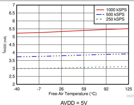
图 5-29. Analog Supply Current vs Temperature
