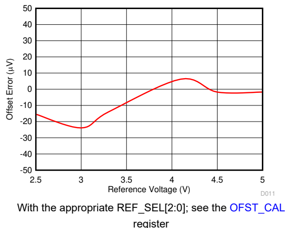
图 5-15. Offset Error vs Reference Voltage
