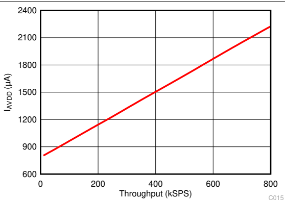
图 5-21. Analog Supply Current vs Throughput
