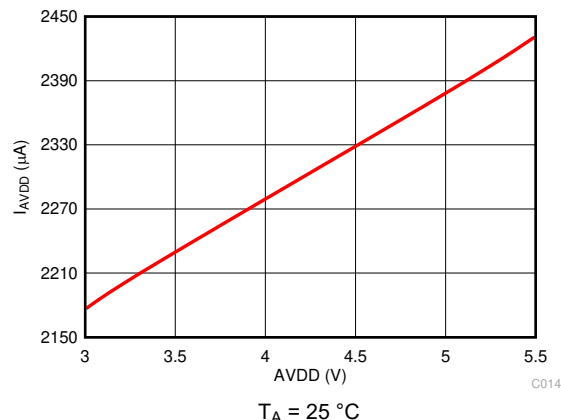
图 5-20. Analog Supply Current vs AVDD
