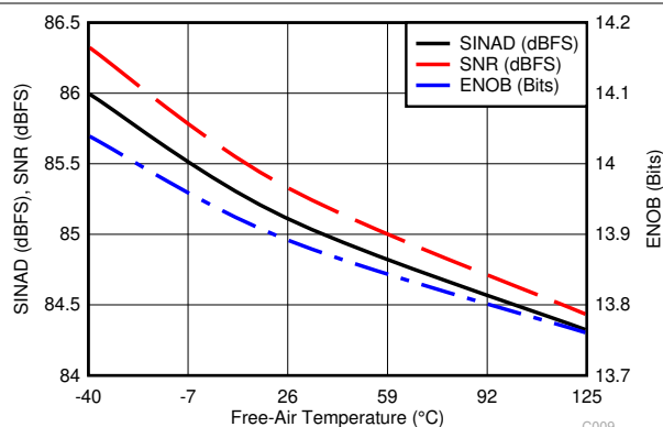
图 5-15. Noise Performance vs Temperature
