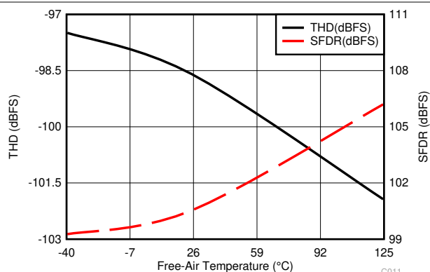
图 5-16. Distortion Performance vs Temperature
