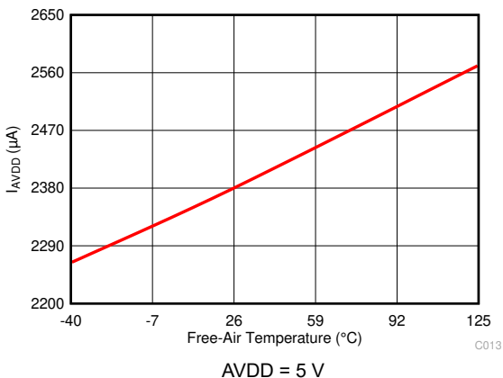
图 5-19. Analog Supply Current vs Temperature
