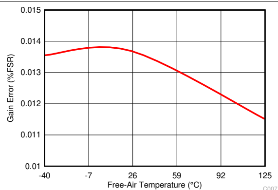
图 5-10. Gain Error vs Temperature
