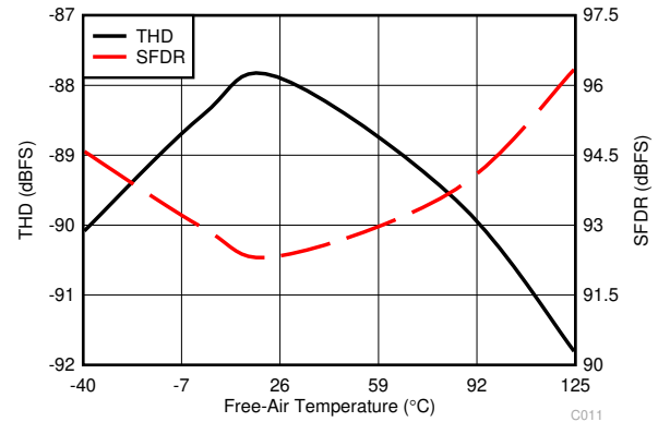
图 6-16. Distortion Performance vs Temperature
