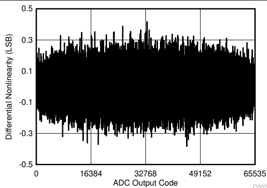
图 6-3. Typical DNL
