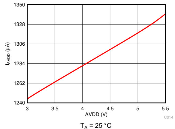
图 6-20. Analog Supply Current vs AVDD
