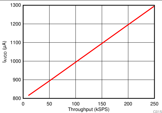
图 6-21. Analog Supply Current vs Throughput
