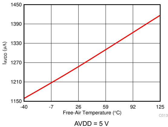
图 6-19. Analog Supply Current vs Temperature
