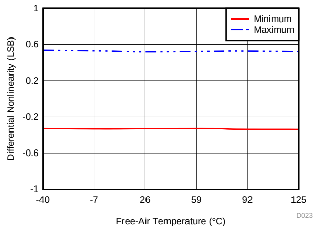
Figure 15. Typical DNL
