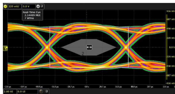
图 7-29. Eye at 7.5-Gbps Bit Rate with Increased Output Swing
