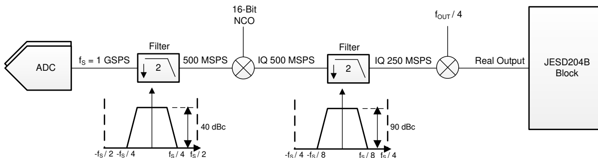
图 7-13. Operating Mode 4
