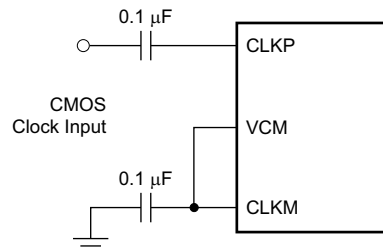
Figure 54. Typical LVCMOS Clock Driving Circuit
