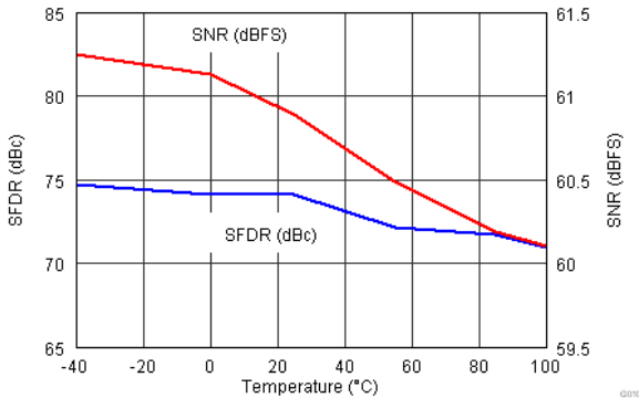
图 7-20. Performance Across Temperature (fin = 230 MHz)
