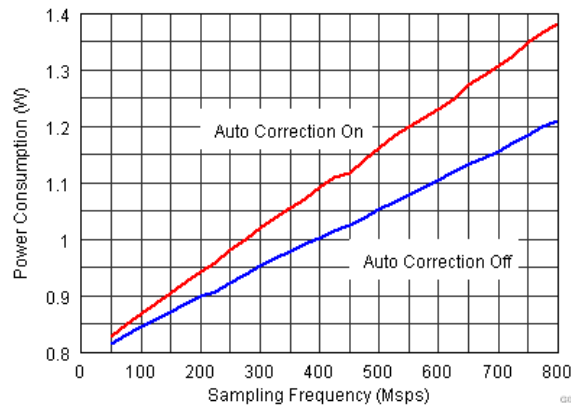
图 7-28. Power Across Sampling Frequency
