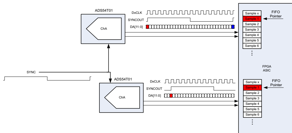
图 8-12. Multi Device SYNC
