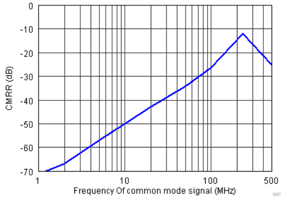
图 7-26. CMRR Across Frequency
