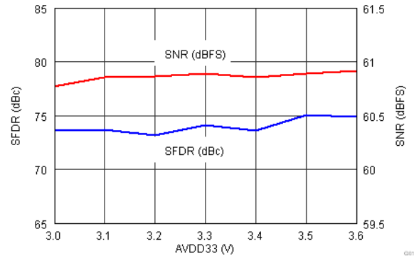
图 7-21. Performance Across AVDD33 (fin = 230 MHz)
