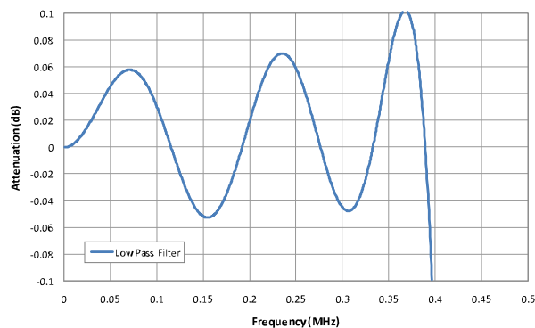
图 8-16. Decimation Filter Response
