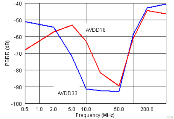
图 7-27. PSRR Across Frequency
