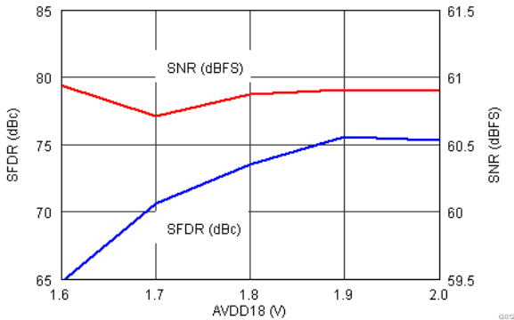
图 7-22. Performance Across AVDD18 (fin = 230 MHz)
