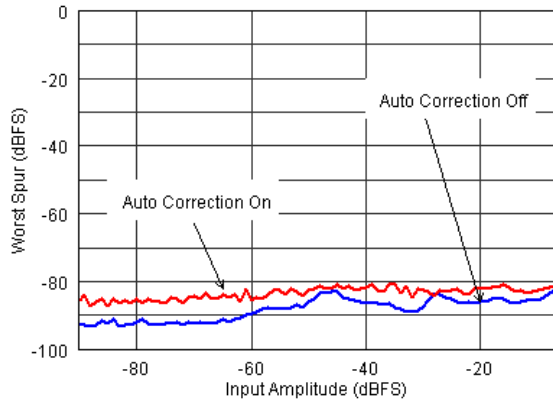
图 7-14. Tow Tone Performance Across Input Amplitude ( f_{\text{in}} = 185 \text{ MHz} )
