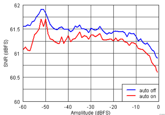
图 7-13. SNR vs. Amplitude (fin = 230 MHz)
