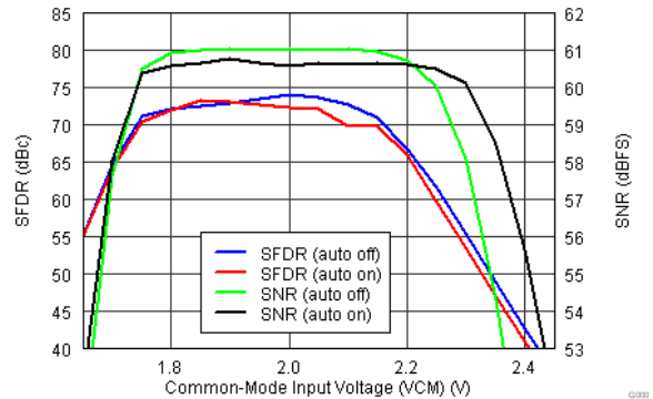
图 7-19. Performance Across Input Common-Mode Voltage
