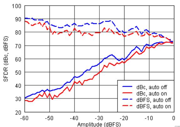
图 7-12. SFDR vs. Amplitude (fin = 230 MHz)
