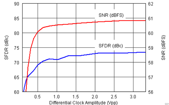
图 7-23. Performance Across Clock Amplitude
