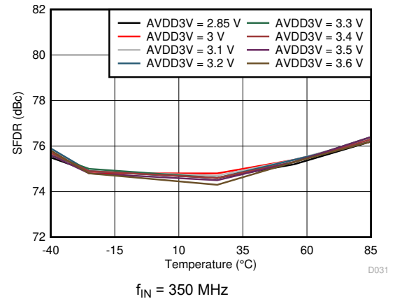
图 7-34. Spurious-Free Dynamic Range vs AVDD3V Supply and Temperature
