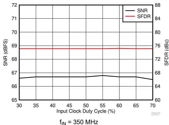
图 7-43. Performance vs Input Clock Duty Cycle
