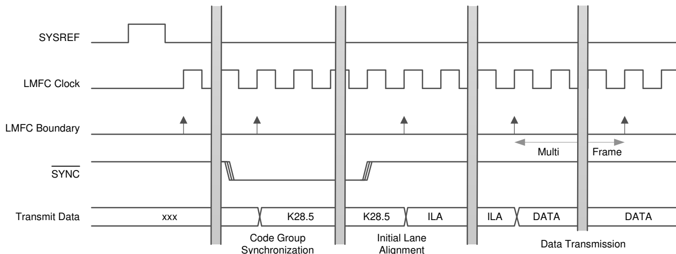
图 8-21. Lane Alignment Sequence
