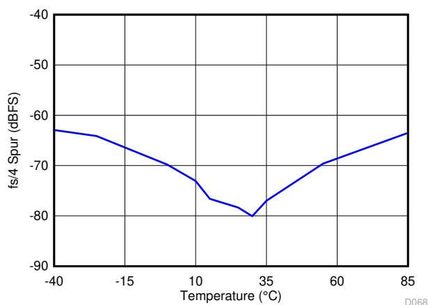
图 9-5. Variation of the f_S / 4 Spur Over Temperature
