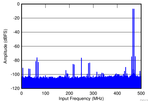
图 7-15. FFT for Two-Tone Input Signal ( -7 dBFS)
