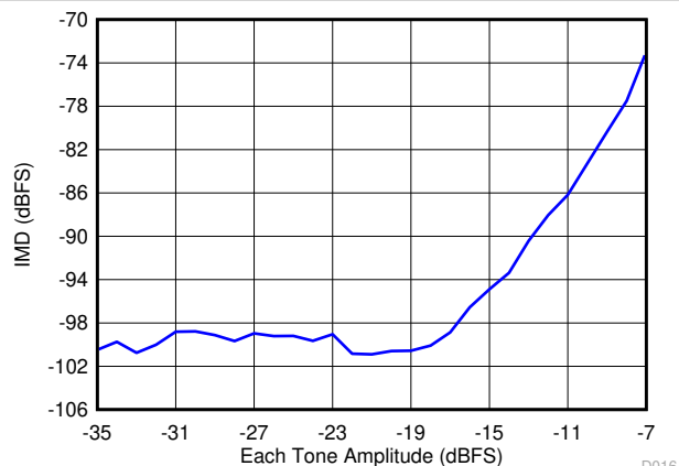
图 7-17. Intermodulation Distortion vs Input Tone Amplitude
