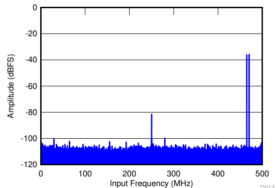
图 7-16. FFT for Two-Tone Input Signal ( -36 dBFS)
