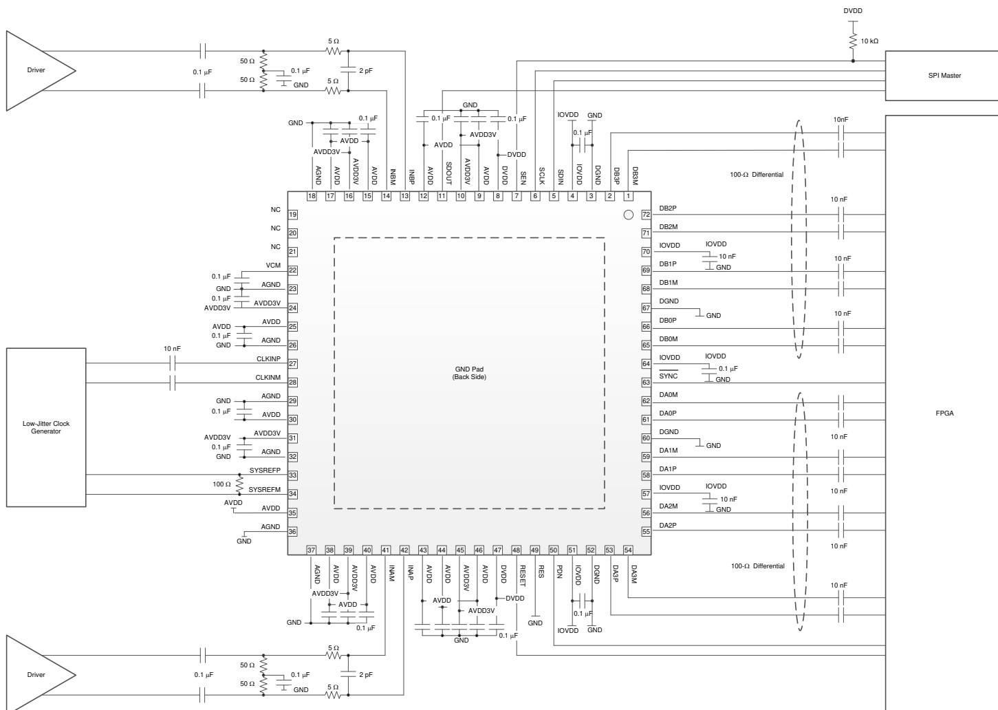
图 9-14. AC-Coupled Receiver
