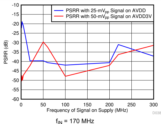
图 7-44. Power-Supply Rejection Ratio vs Test Signal Frequency
