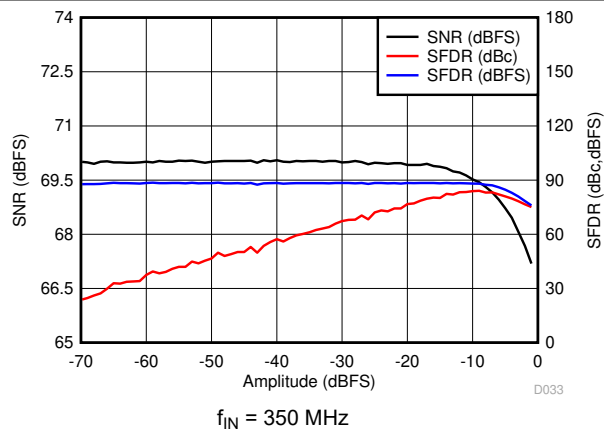
图 7-39. Performance vs Input Amplitude
