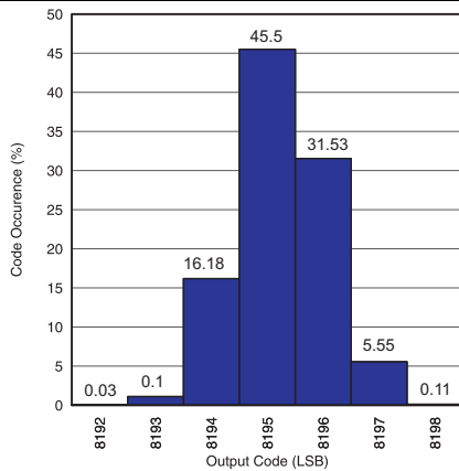
图 28. Histogram of Output Code With Analog Inputs Shorted (RMS Noise = 96.4 \mu V) a note "RMS Noise = 96.4 \mu V" to 图 28
