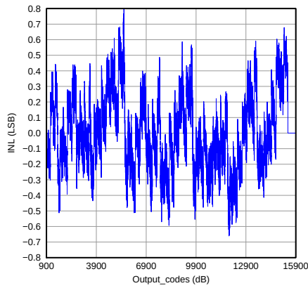
图 26. Integral Non-Linearity
