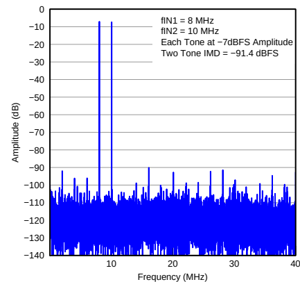
图 13. Two-Tone Intermodulation
