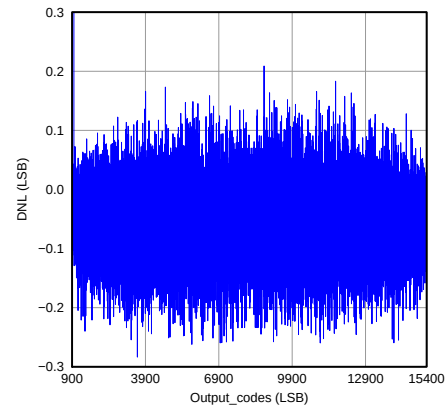
图 27. Differential Non-Linearity
