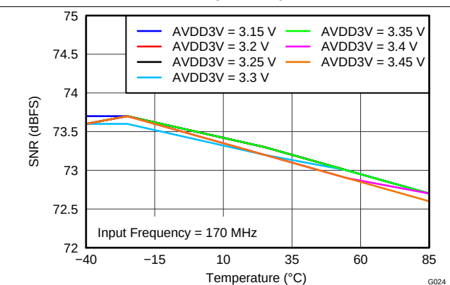
Figure 22. SNR vs AVDD Supply and Temperature (170 MHz)
